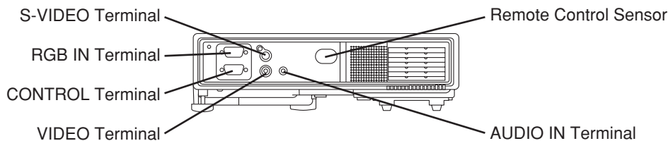
TERMINAL PANEL
