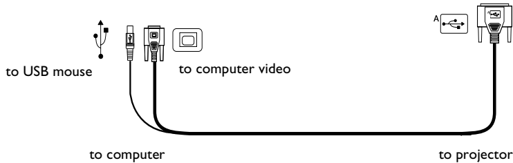
FIGURE 5 Computer cable
