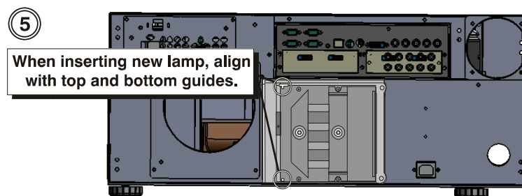
Figure 4.5. Insert New Lamp Module
