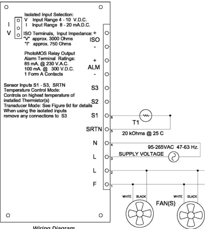
Wiring Diagram
