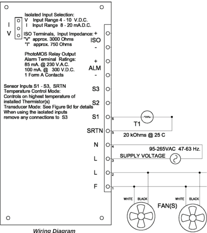
Wiring Diagram
