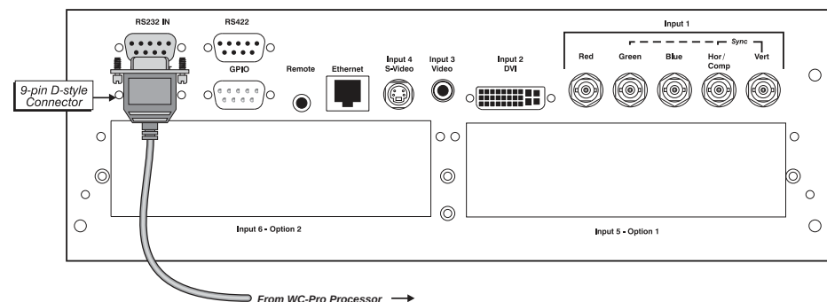
Figure 2.10 Connecting RS-232
