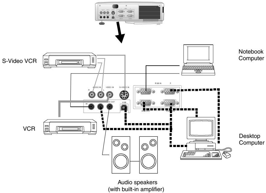
Figure 3: System Setup
