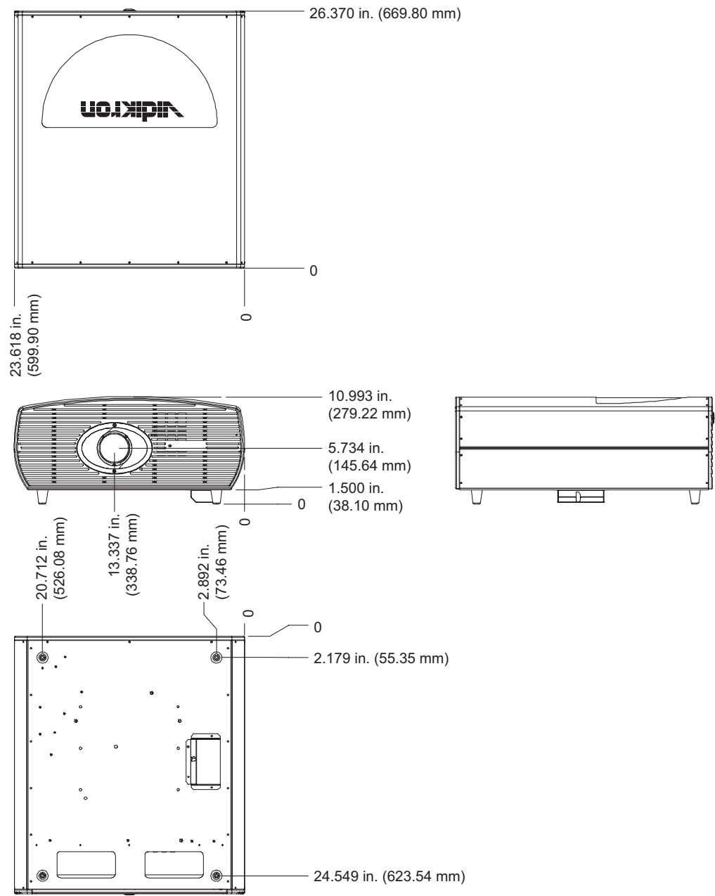
Figure 7-1. Vision 90 Dimensions
