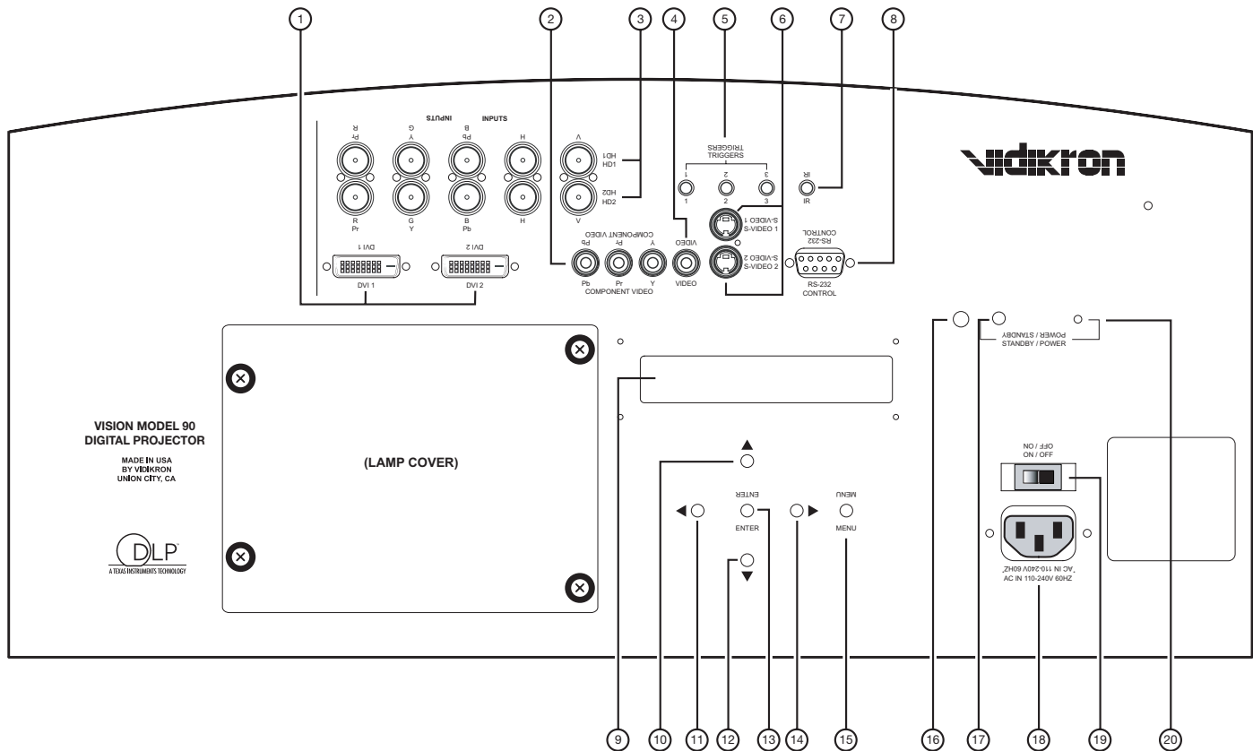
Figure 2-2. Vision 90 Rear Panel
