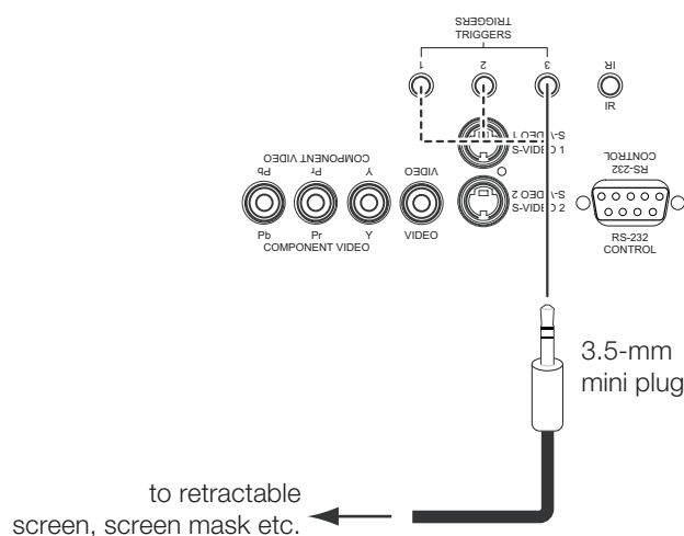
Figure 3-12. Connecting 12-Volt Trigger Outputs
