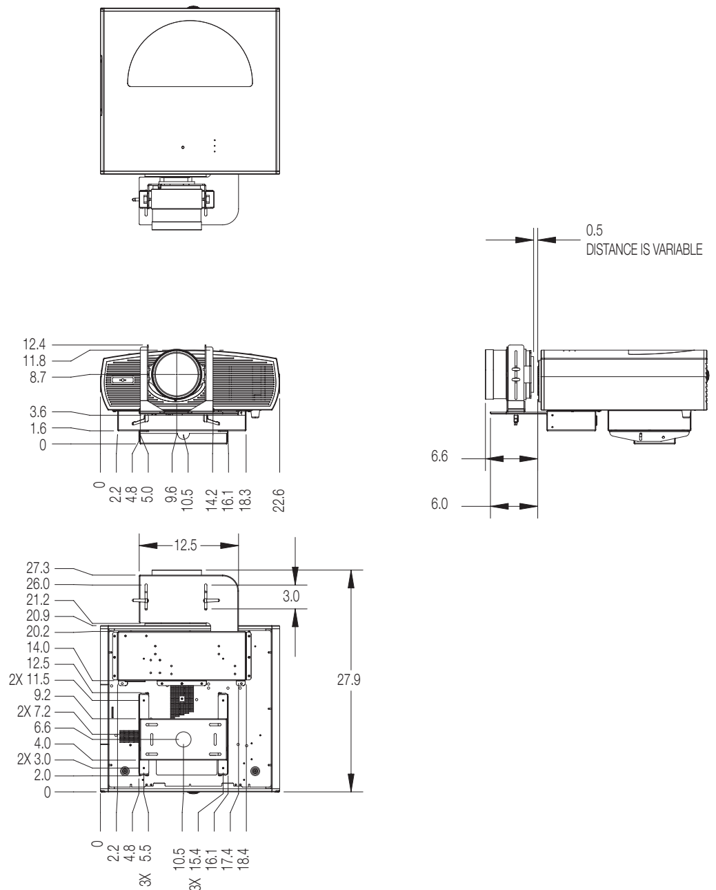
Figure 7-1. Vision 85/CineWide with AutoScope Dimensions
