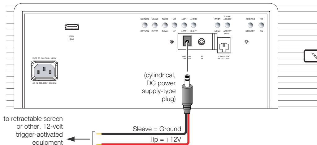
Figure 3-17. 12-volt Trigger Output Connection (from Projector)
