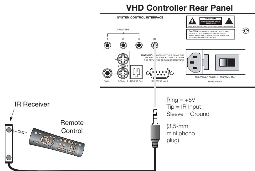
Figure 3-18. External IR Receiver Connection
