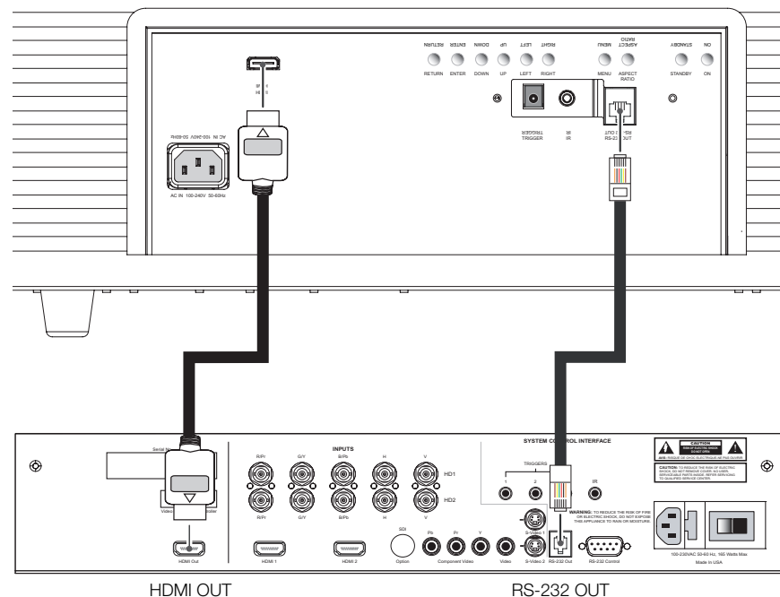
Figure 3-10. Connecting the Projector to the VHD Controller
