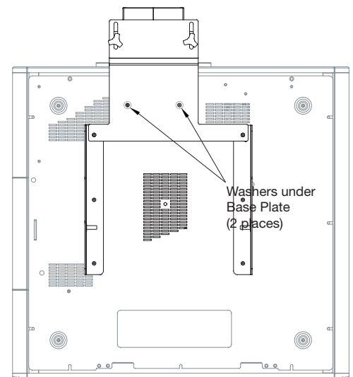
Figure 3-9. Vision 85/CineWide with Anamorphic Lens Base Plate and Ceiling Mounting Rails - Bottom View
