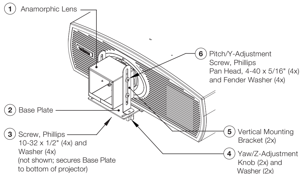
Figure 3-20. Vision 85 Anamorphic Lens Mounting Assembly - Exploded View
