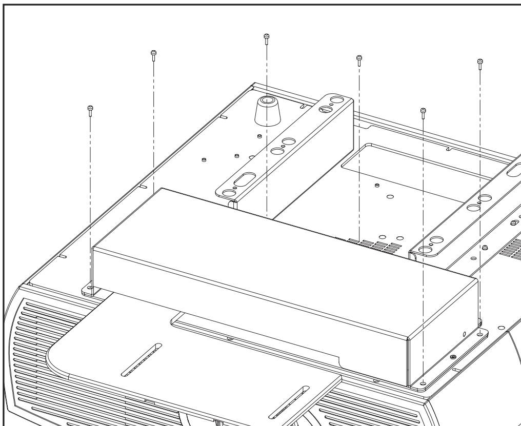
Figure 3-8. AutoScope Lens Motor Installation
