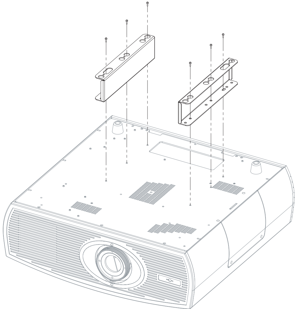
Figure 3-7. Vision 85 with Ceiling Mount Adapters/Projector Stands
