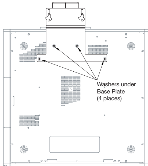
Figure 3-9. Vision 85/CineWide with Anamorphic Lens Base Plate and Ceiling Mounting Rails - Bottom View
