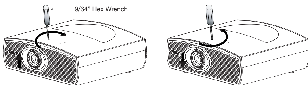
Figure 3-19. Vertical Lens Shift Adjustments
