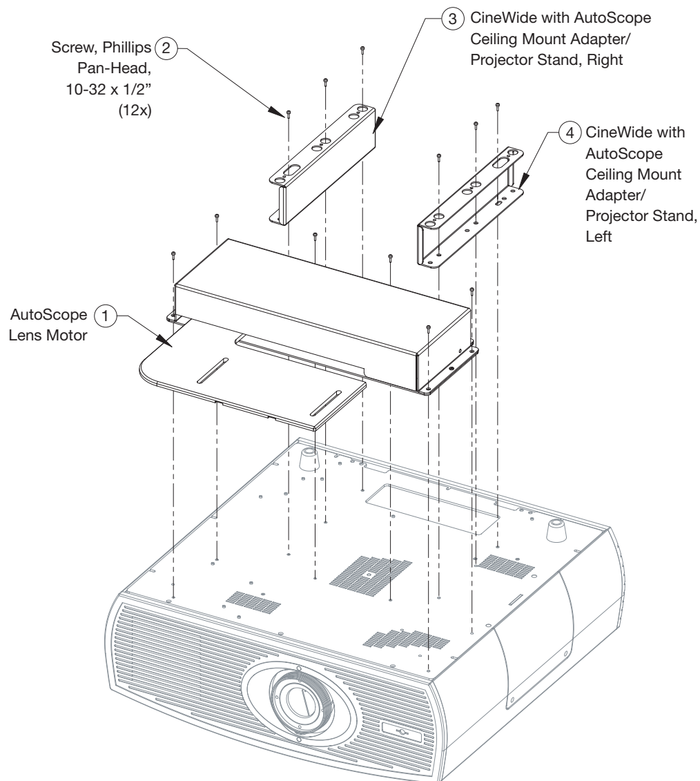
Figure 3-6. Vision 85/CineWide with AutoScope Motor Assembly – Exploded View
