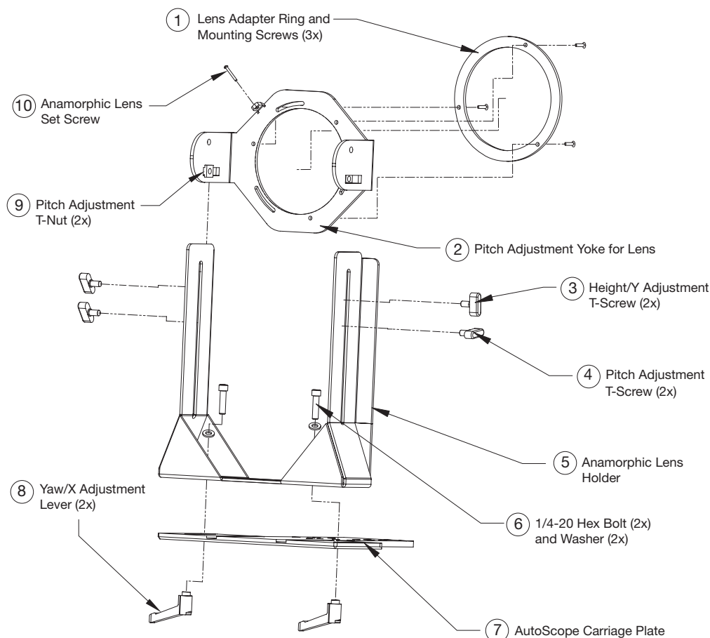
Figure 3-21. Anamorphic Lens Mounting Assembly - Exploded View
