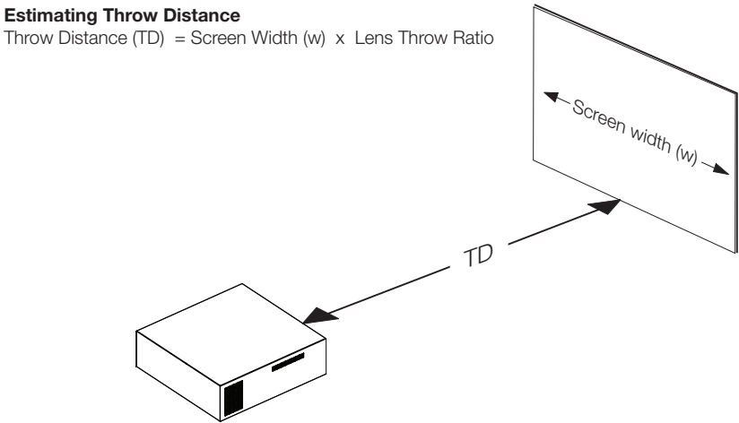
Figure 3-1. Estimating Throw Distance
