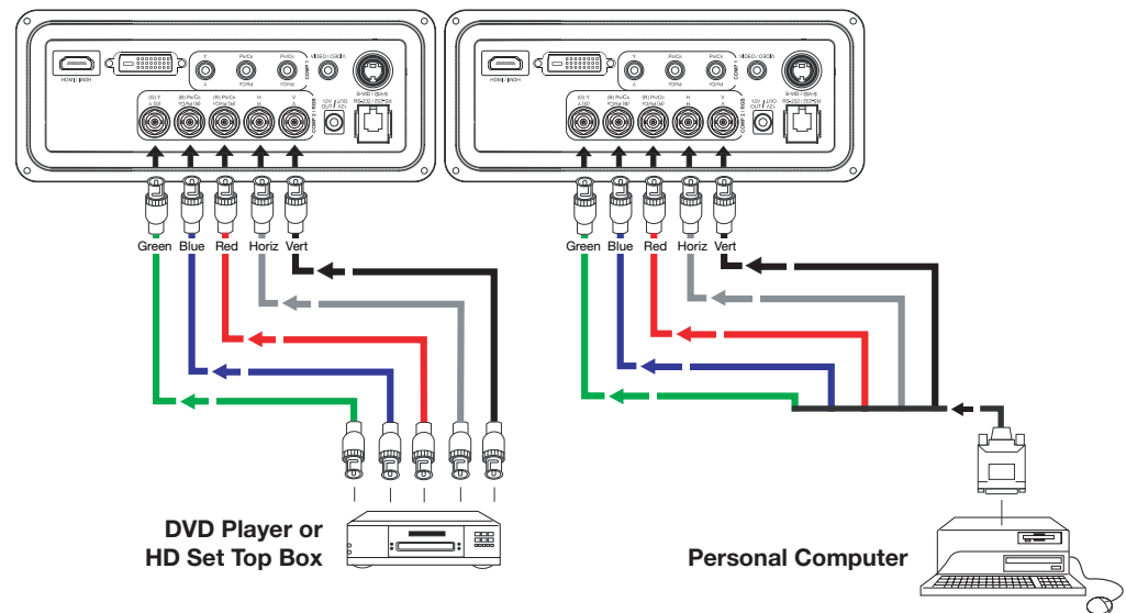
Figure 3-10. RGB Connections
