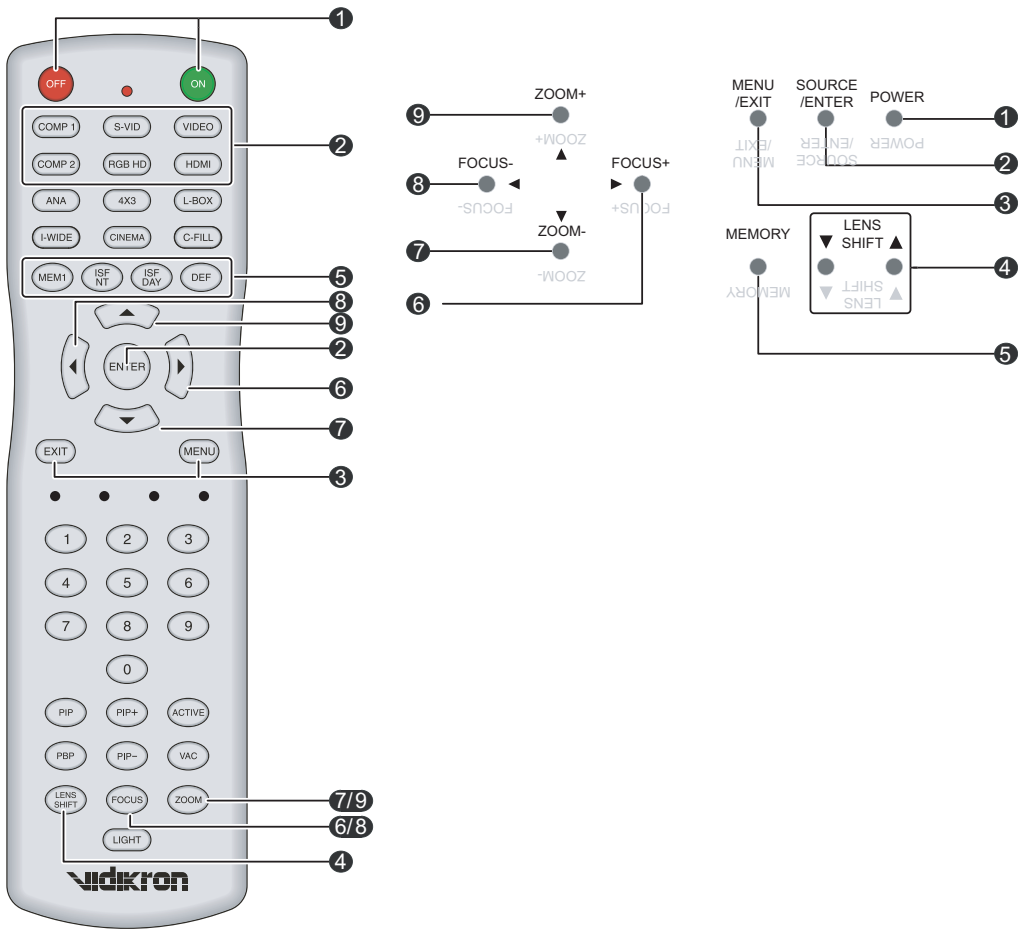
Figure 2-5. Remote Control/Built-In Keypad Functional Cross-Reference
