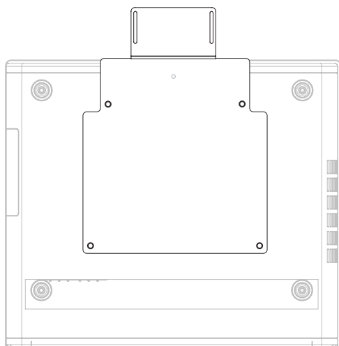
Figure 3-8. Vision 70/CineWide with Anamorphic Lens Base Plate and Ceiling Mounting Plate - Bottom View
