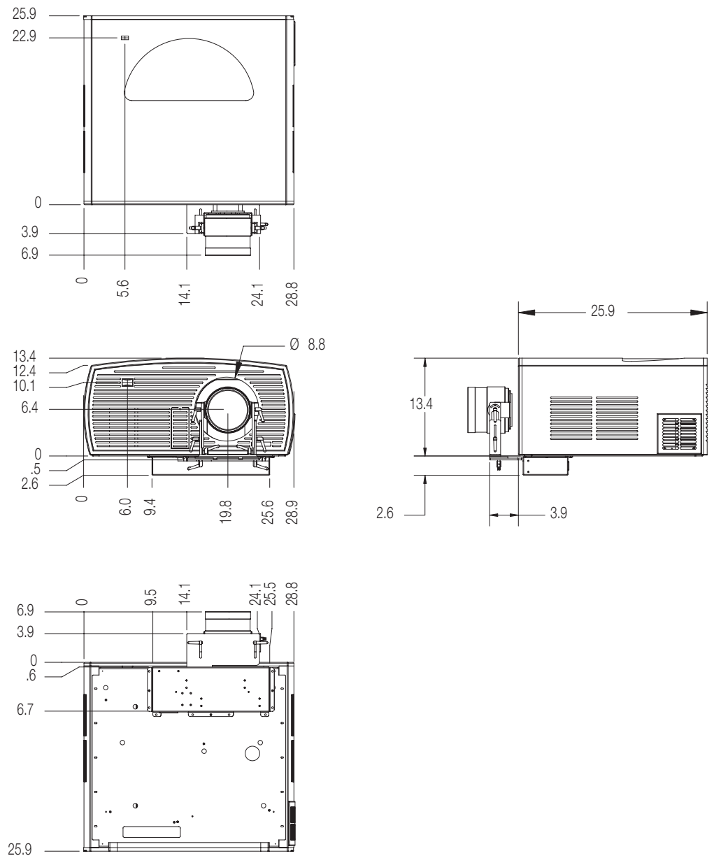
Figure 7-1. Vision 150 Dimensions
