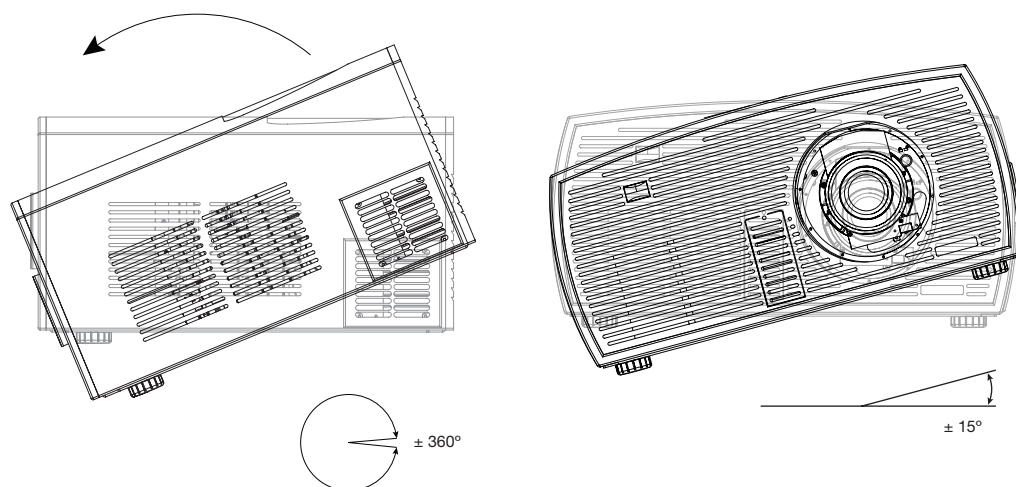
Figure 3-8. Mounting Angle Ranges (Front-to-Back and Side-to-Side)
