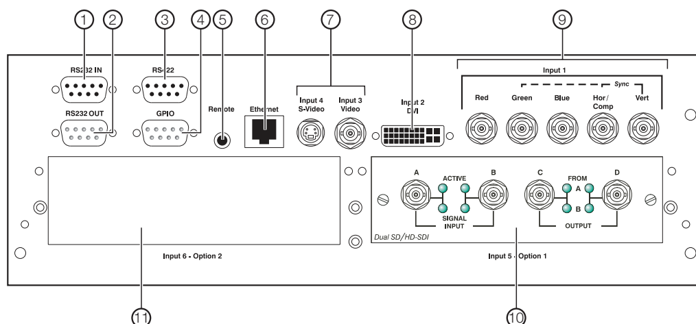
Figure 2-2. Vision 150 Input Panel
