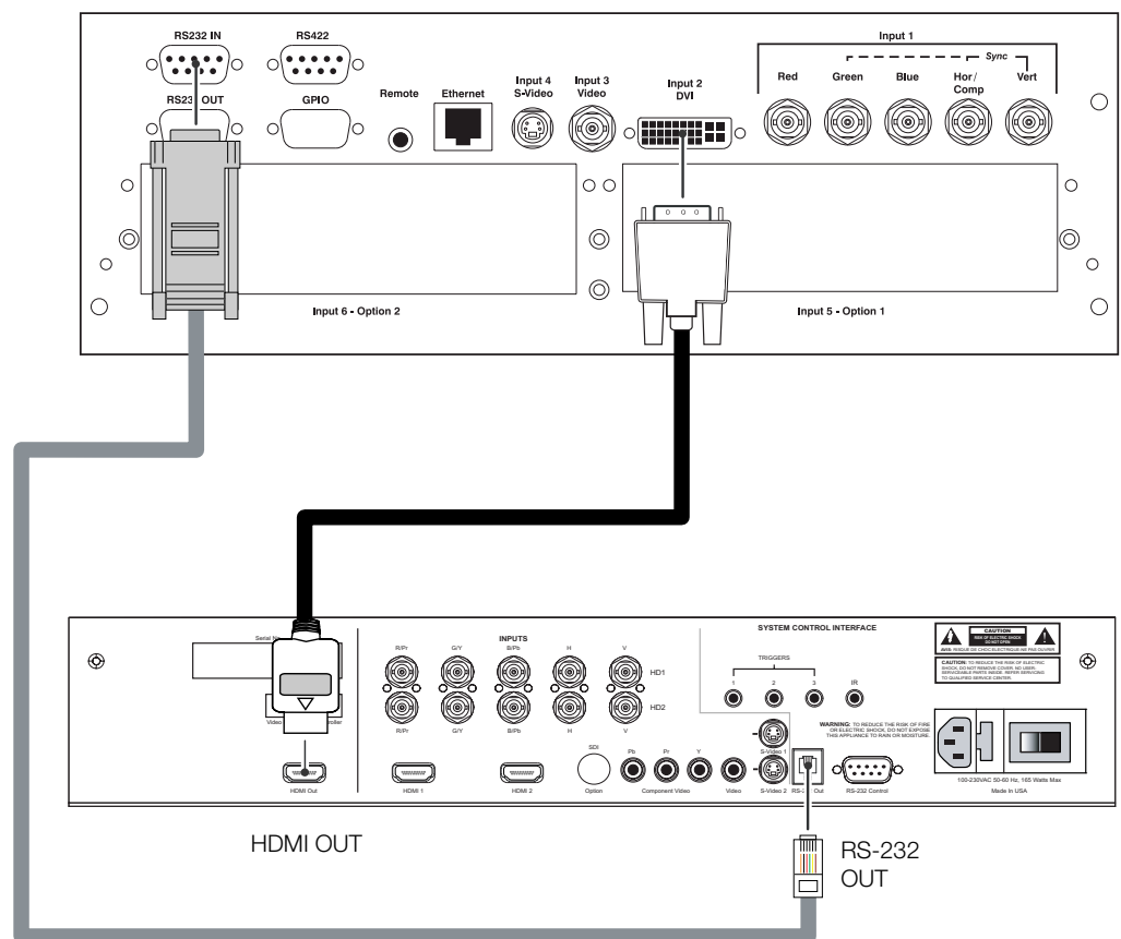
Figure 3-9. Connecting the Vision 150 to the VHD Controller
