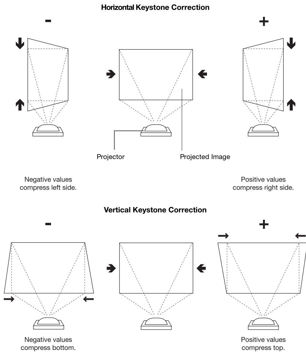
Figure 4-6. Keystone Correction
