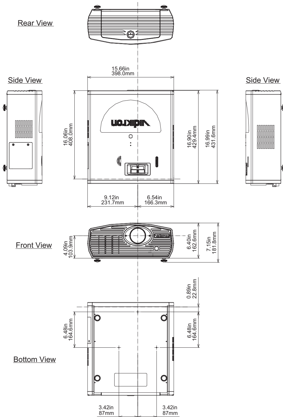
Figure 7-1. Vision 15 Dimensions
