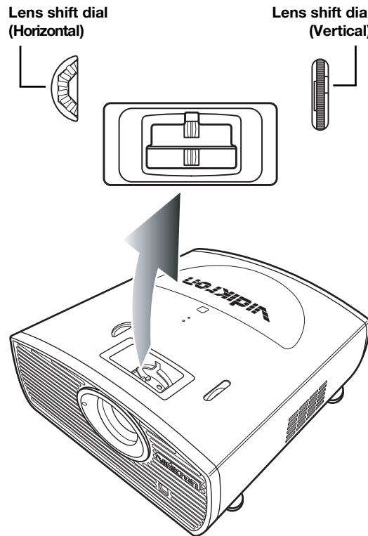
Figure 3-16. Vertical and Horizontal Lens Shift Controls
