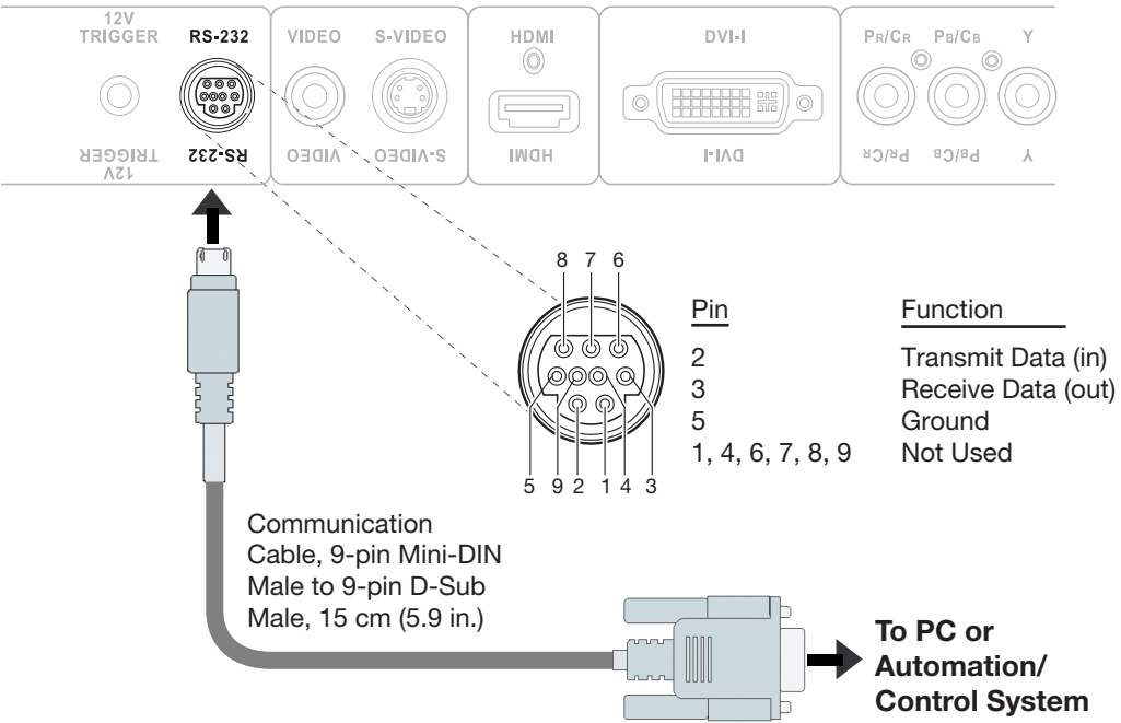
Figure 3-13. RS-232 Control System Connection
