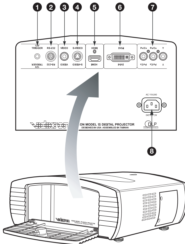
Figure 2-2. Vision 15 Rear Panel
