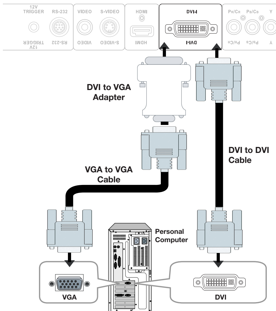
Figure 3-10. RGB Connections
