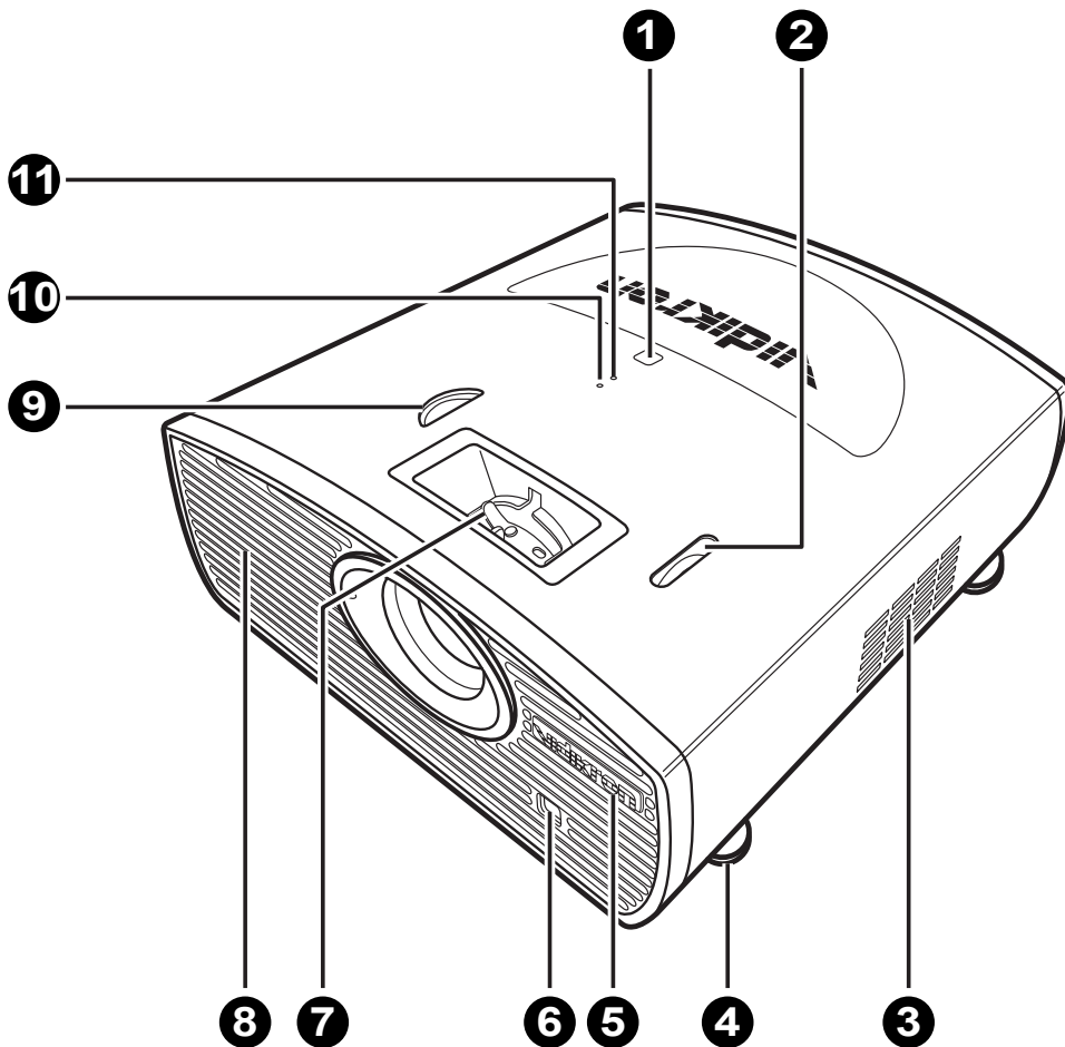
Figure 2-1. Vision 15 Front/Side/Top View
