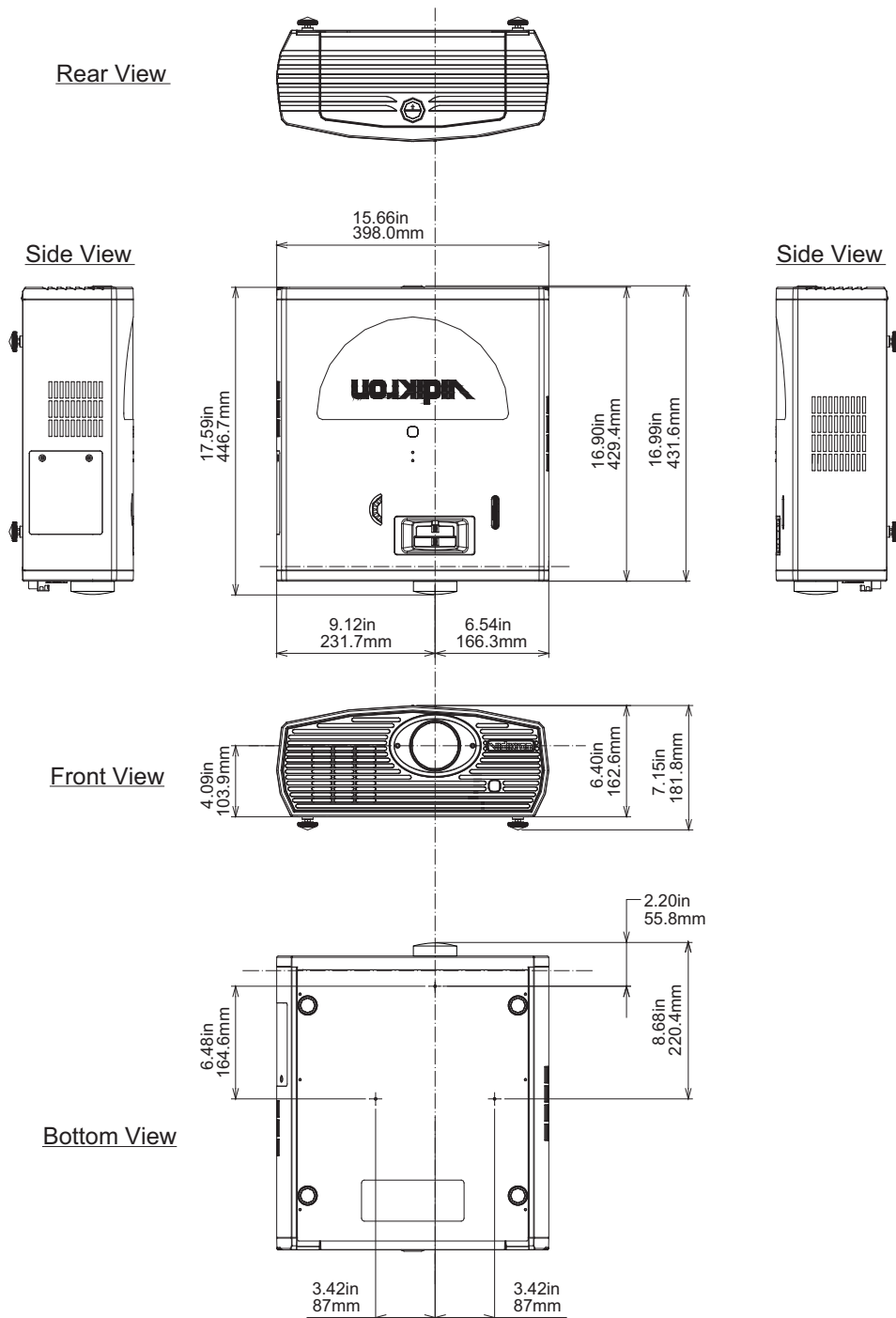
Figure 7-2. Vision 15ET Dimensions
