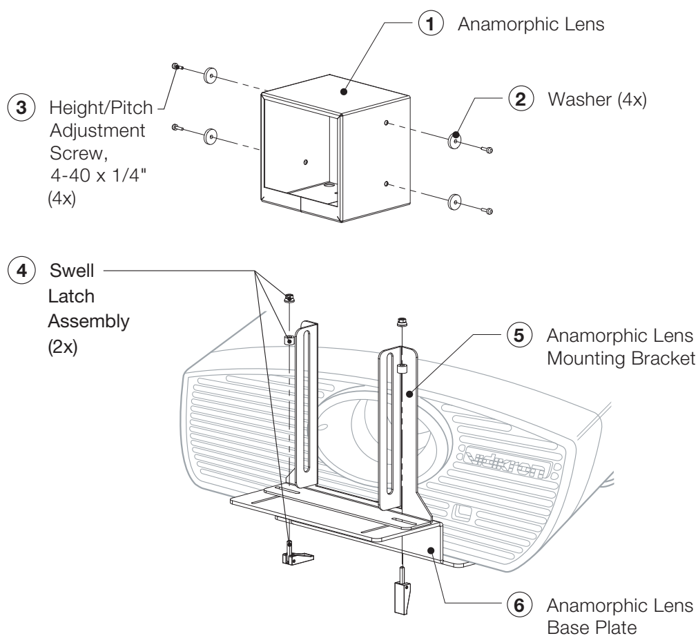
Figure 3-17. Anamorphic Lens Mounting Assembly - Exploded View
