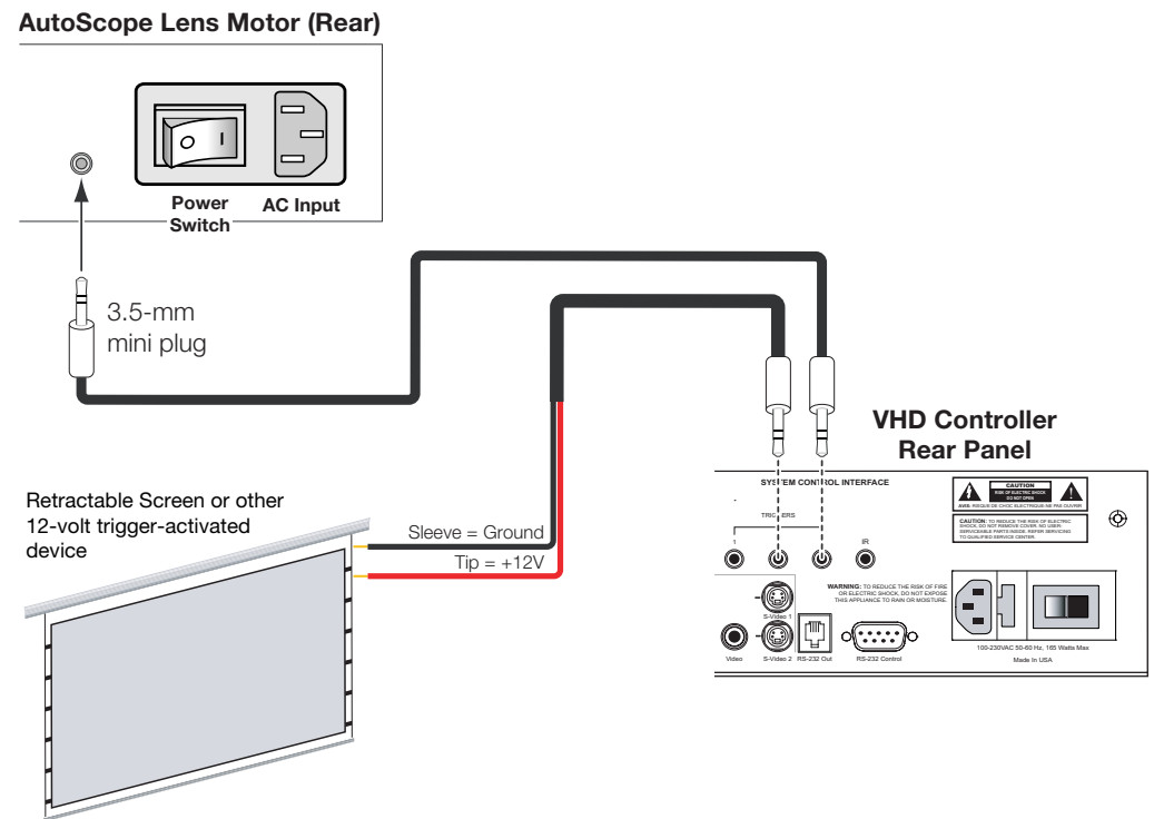
Figure 3-15. Connecting 12-Volt Trigger Outputs
