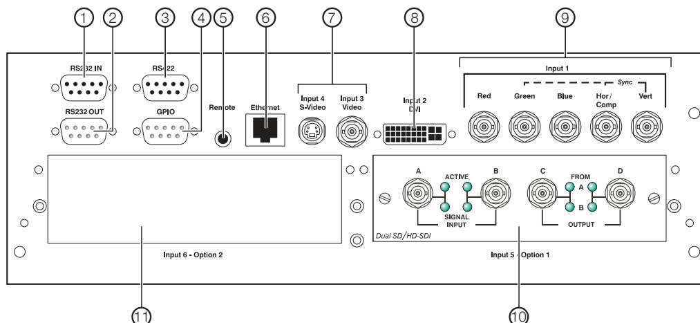
Figure 2-2. Vision 140/150 Input Panel
