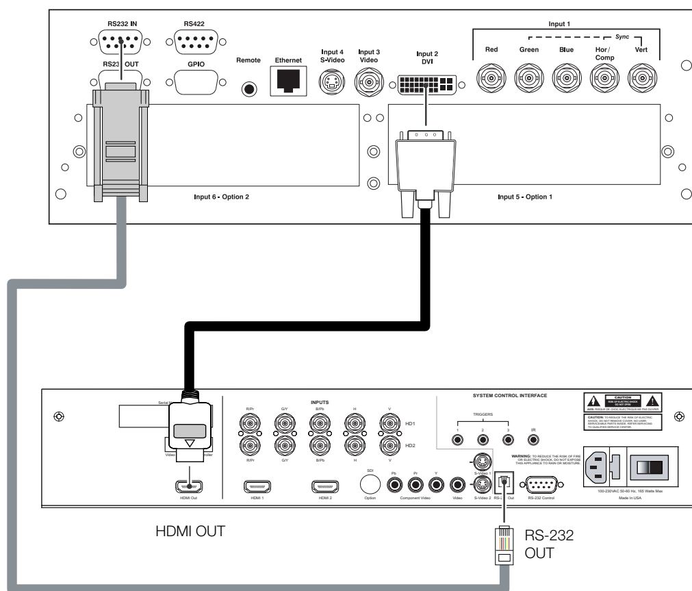
Figure 3-9. Connecting the Vision 140/150 to the VHD Controller
