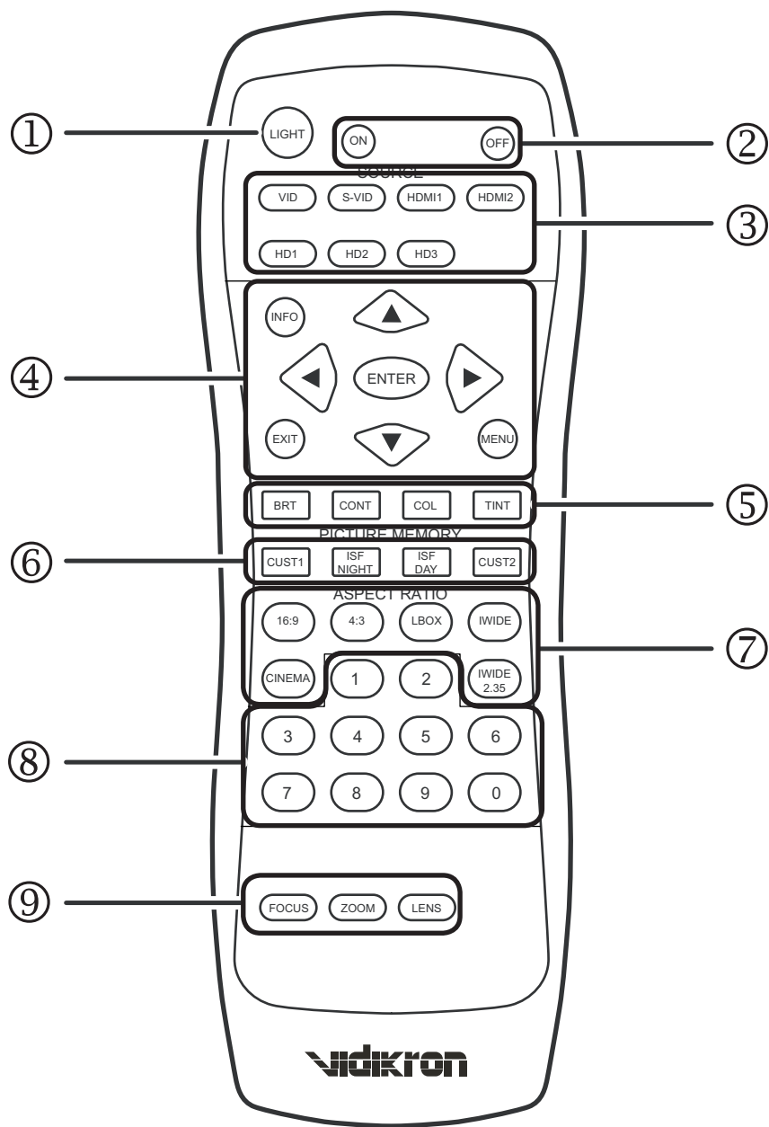
Figure 2-4. Vision 110 Remote Control
