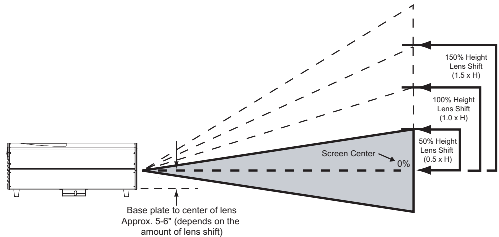
Figure 3-3. Vertical Lens Shift (Example Only)
