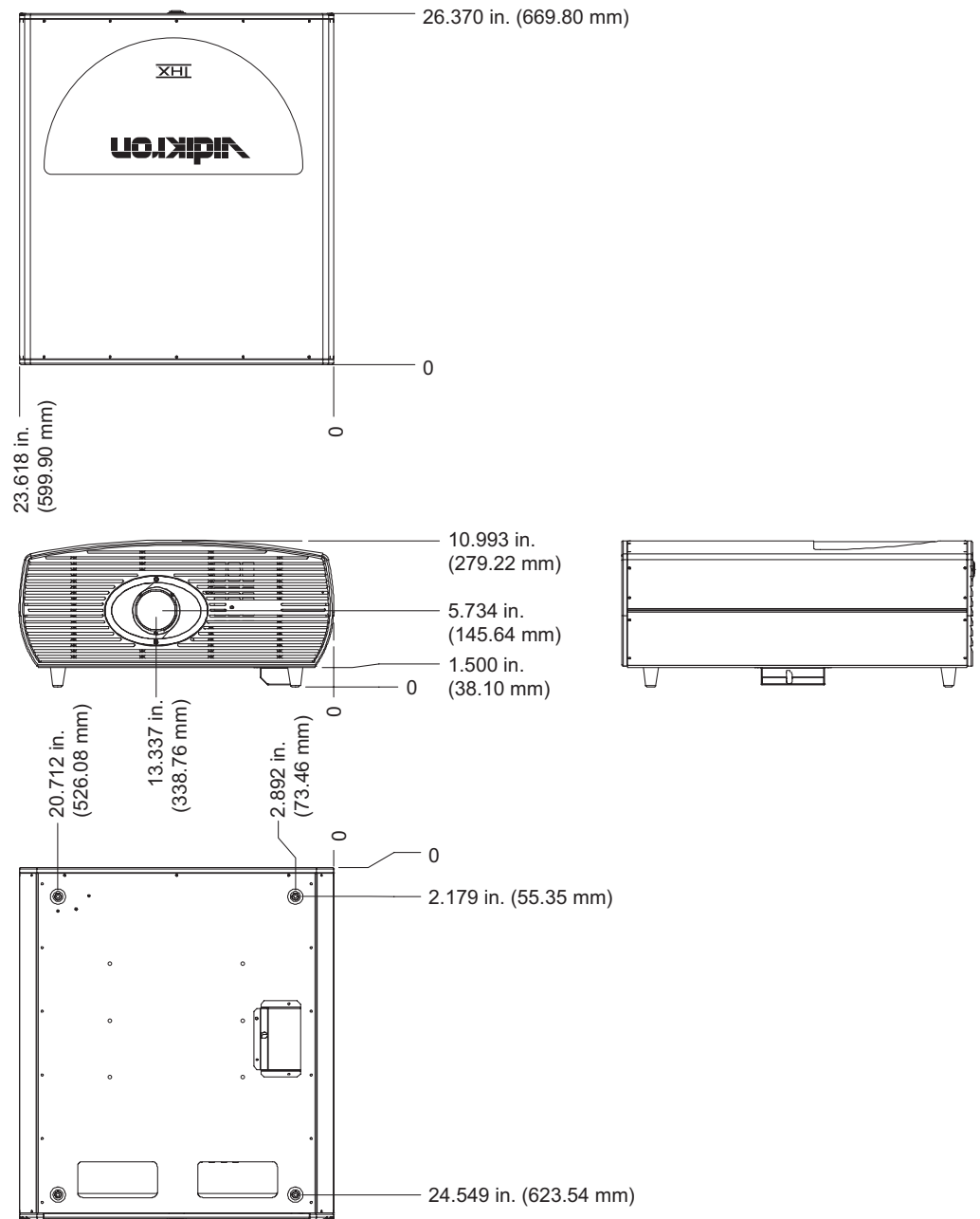
Figure 7-1. Vision 90t/100t Dimensions
