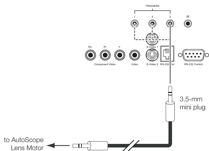
Figure 3-11. Connecting a 12-Volt Trigger Output to the AutoScope Lens Motor
