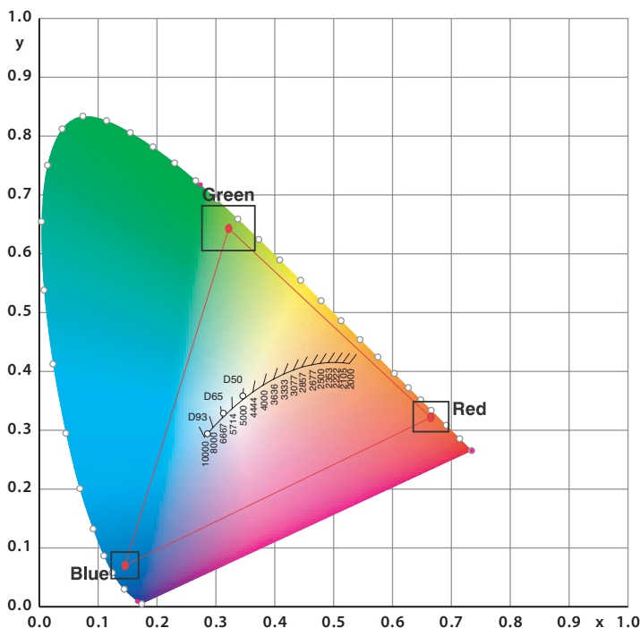
Figure A-1. CIE 1931 Chromaticity Diagram
