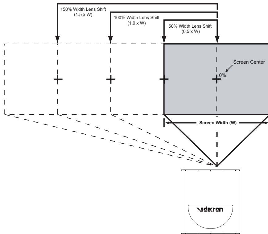
Figure 3-4. Horizontal Lens Shift (Example Only)
