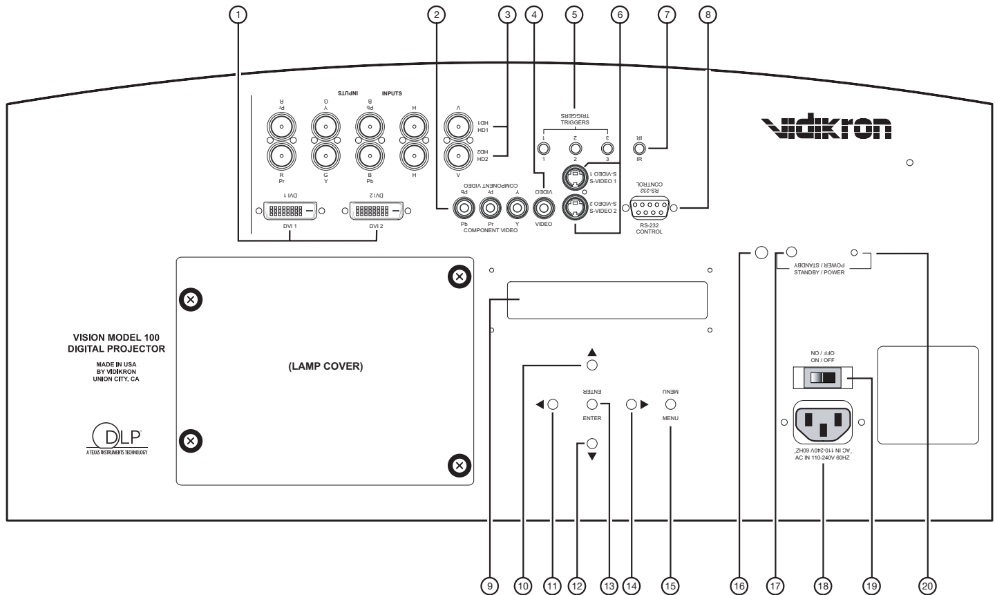
Figure 2-2. Vision 90t/100t Rear Panel
