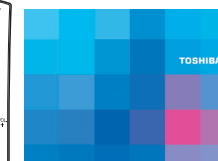
Start-up screen
