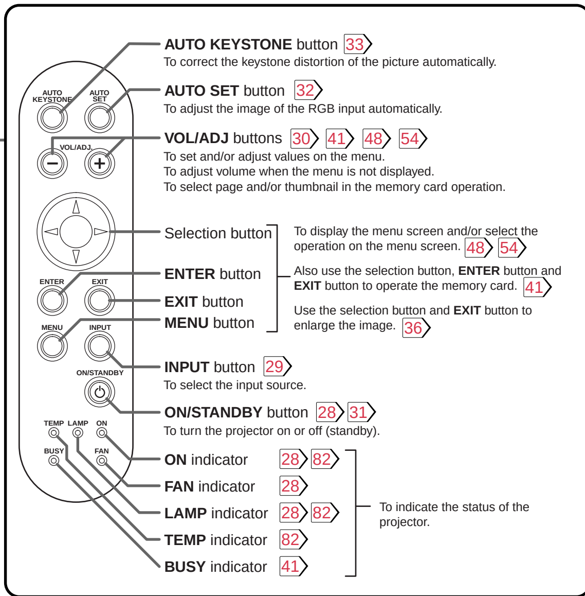
Control panel
