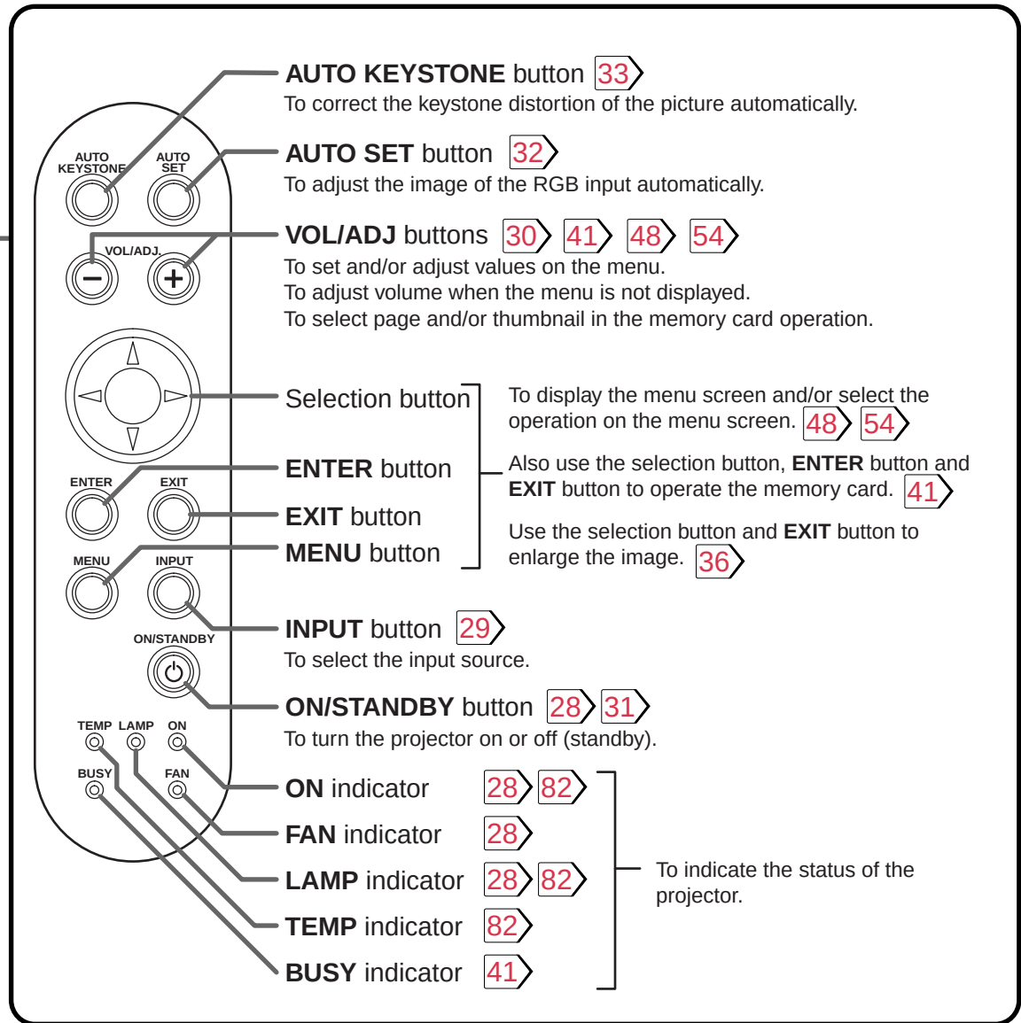
Control panel
