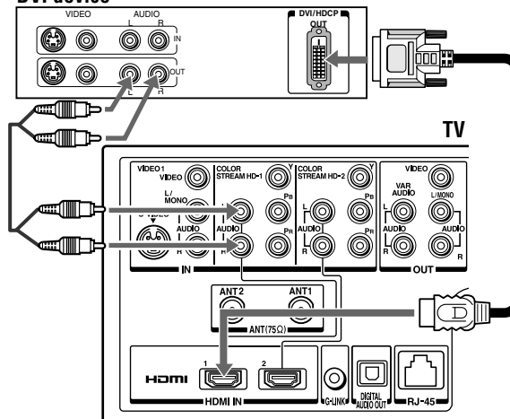
DVI device
