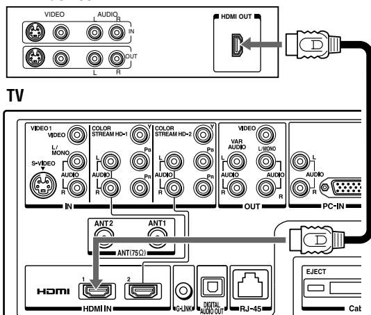
HDMI device
