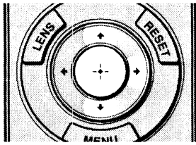
Pop-up menu
