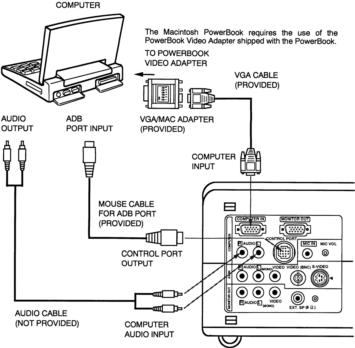
VGA/MAC ADAPTER
