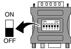
MAC/VGA ADAPTER
