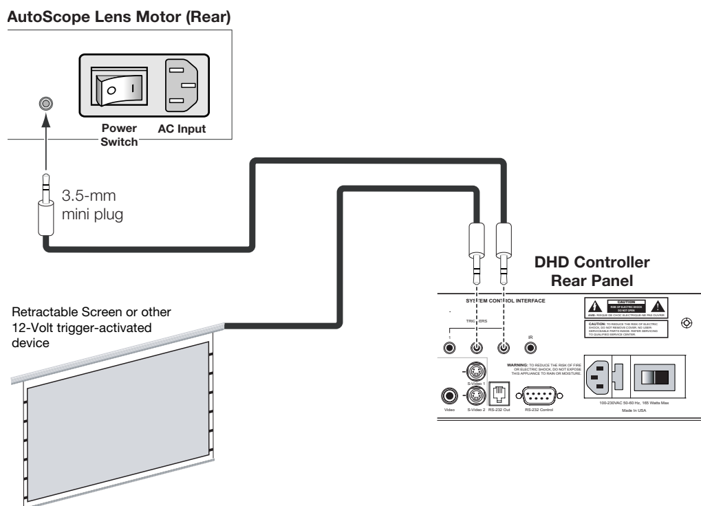
Figure 3-14. Connecting 12-Volt Trigger Outputs
