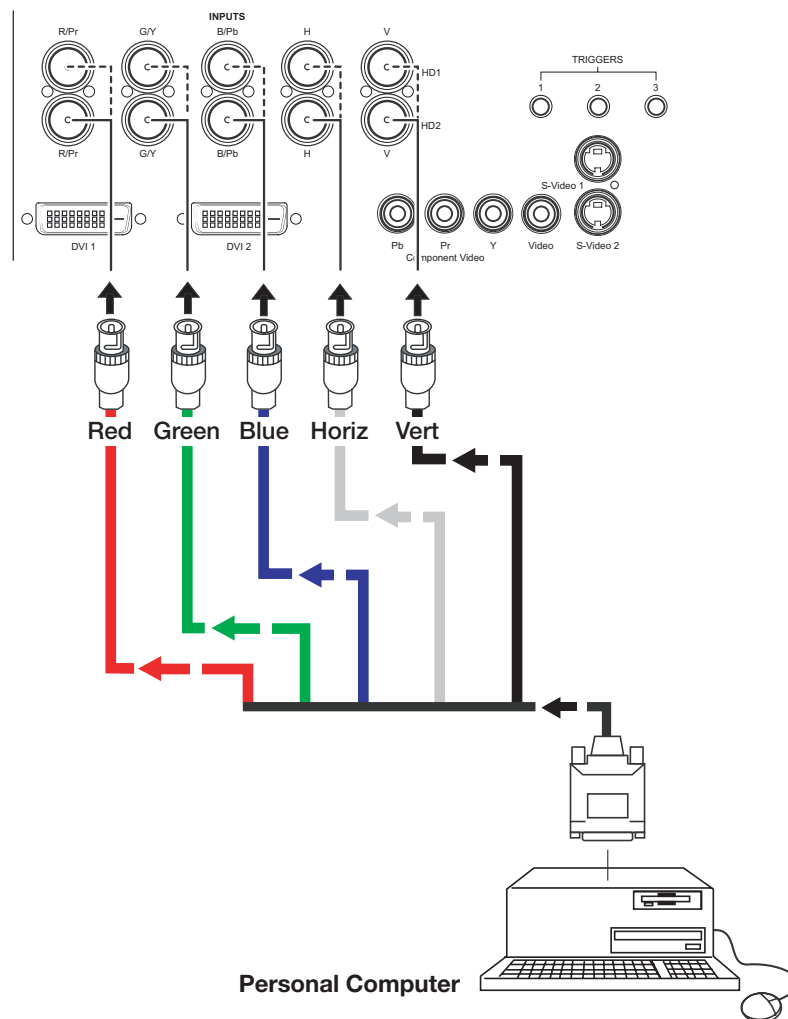
Figure 3-11. Analog RGB Connections
