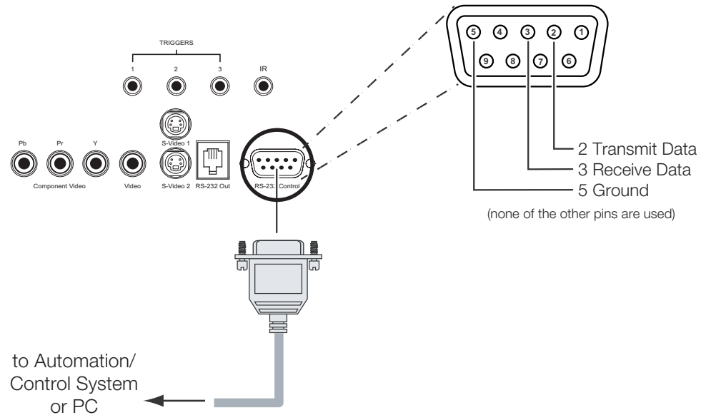
Figure 3-13. RS-232 Control System Connection
