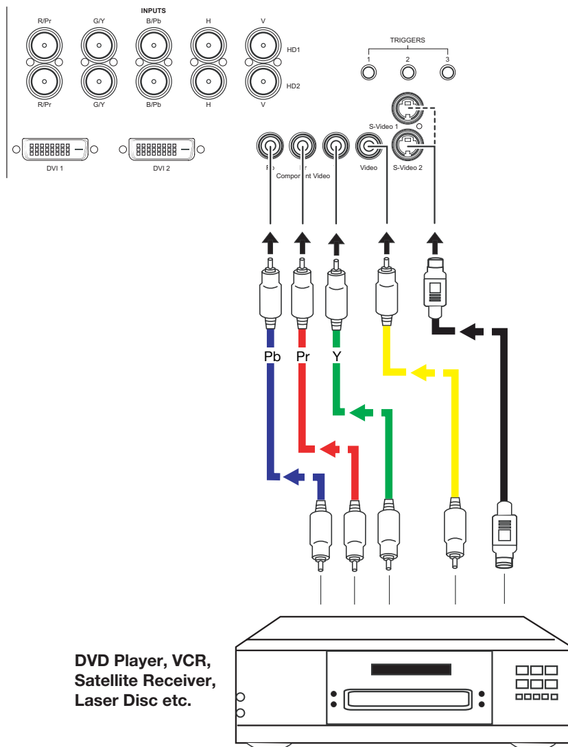
Figure 3-12. Composite, S-Video and Component Video Connections
