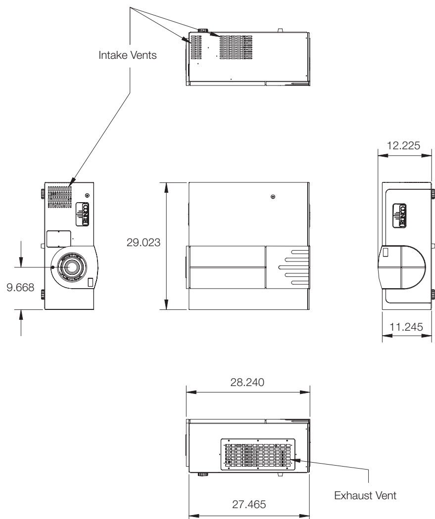
Figure 7-1. VX-40d/-50d/-60d/-80d Dimensions
