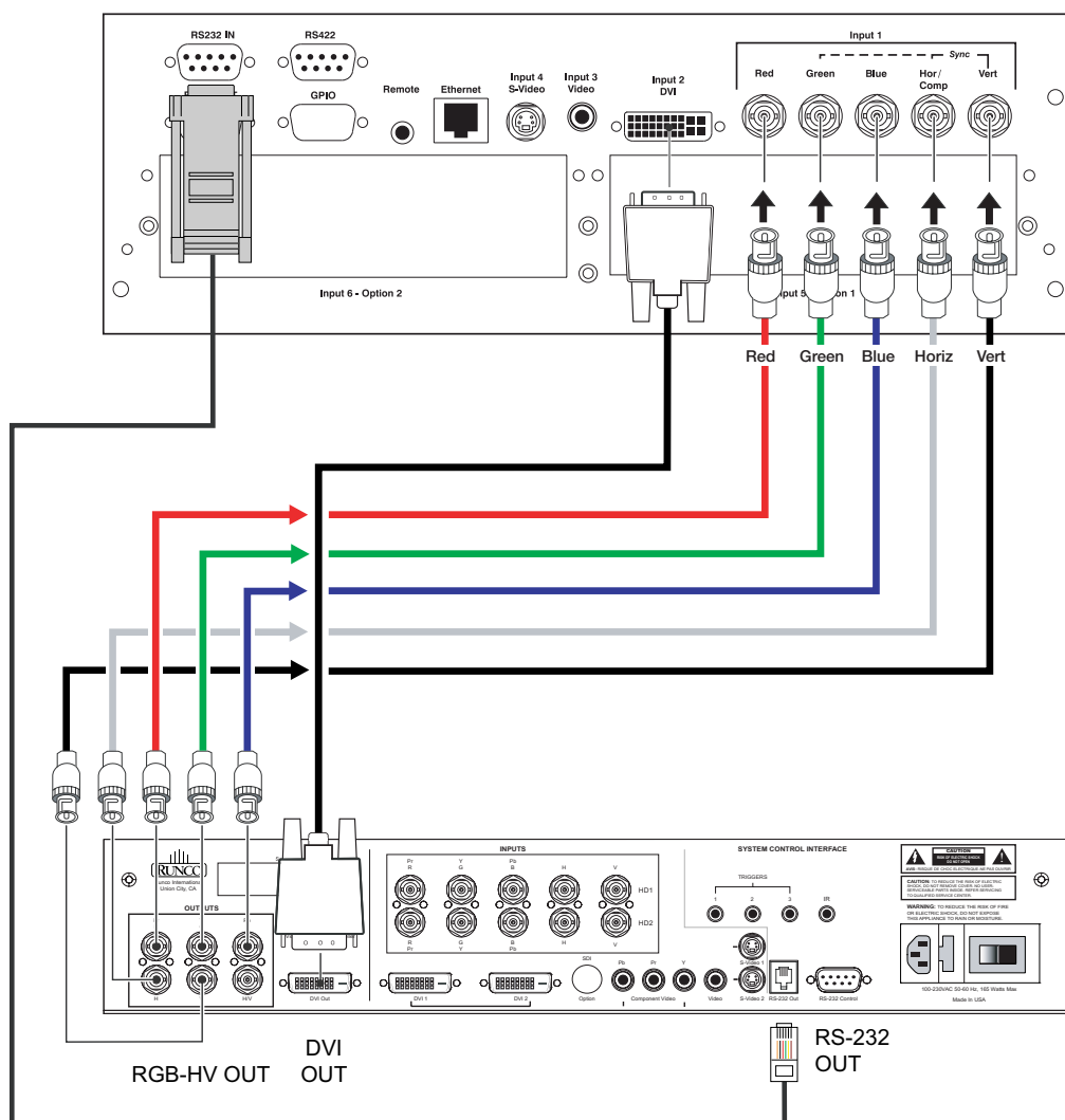
Figure 3-8. Connecting the VX-40d/-50d/-60d/-80d to the DHD Controller
