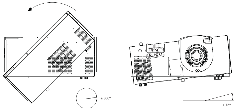
Figure 3-7. Mounting Angle Ranges (Front-to-Back and Side-to-Side)
