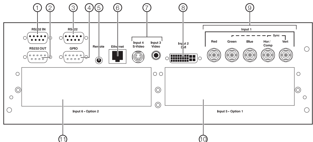
Figure 2-2. VX-40d/-50d/-60d/-80d Input Panel
