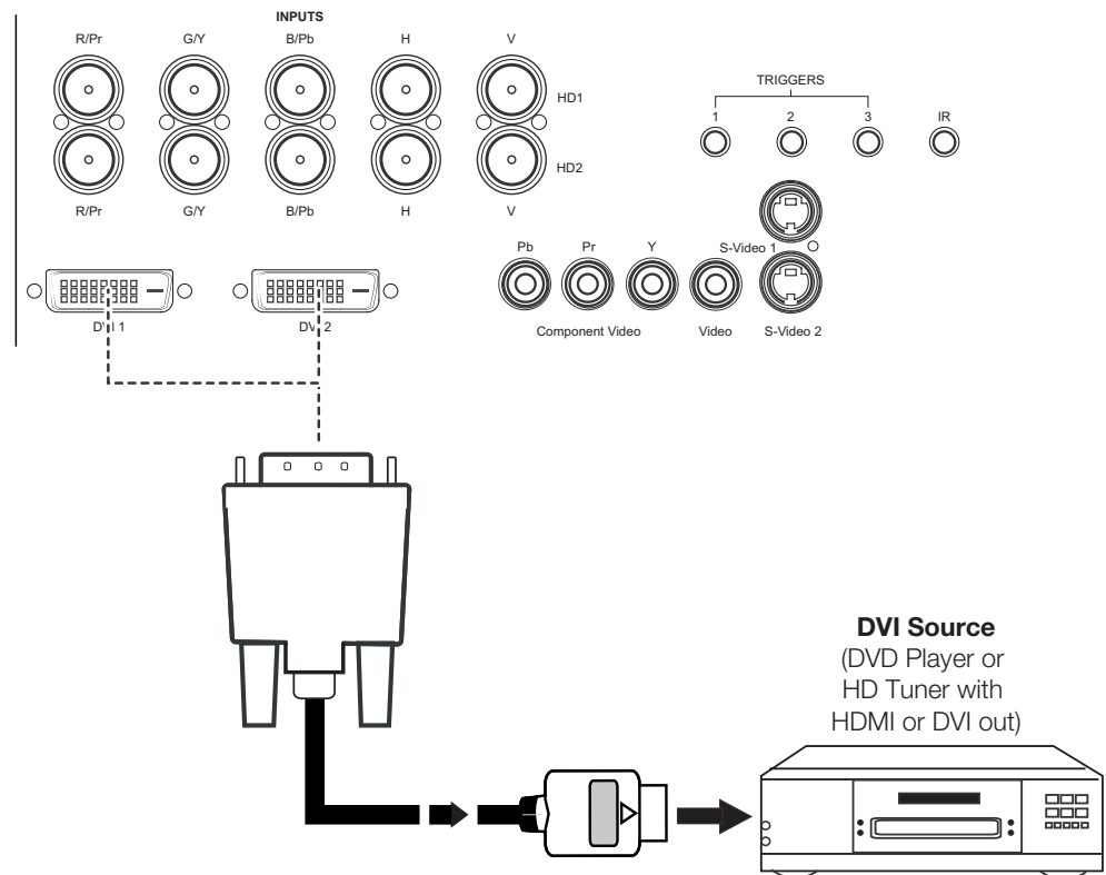
Figure 3-9. DVI Source Connections
