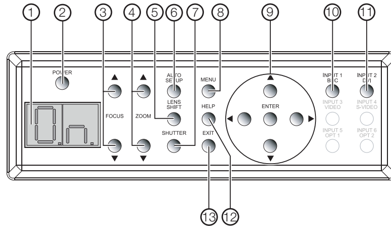
Figure 2-3. VX-40d/-50d/-60d/-80d Rear-Panel Keypad
