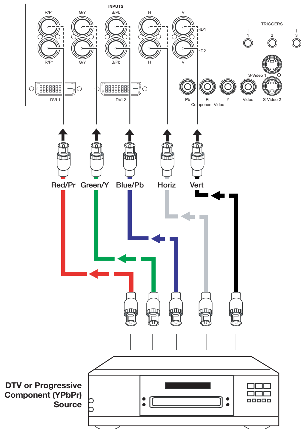
Figure 3-10. Digital (DTV) RGB or Component Video Connections
