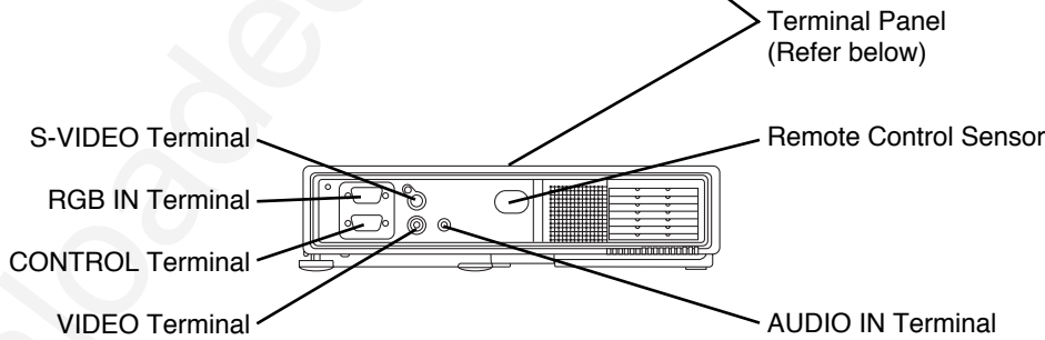
TERMINAL PANEL
