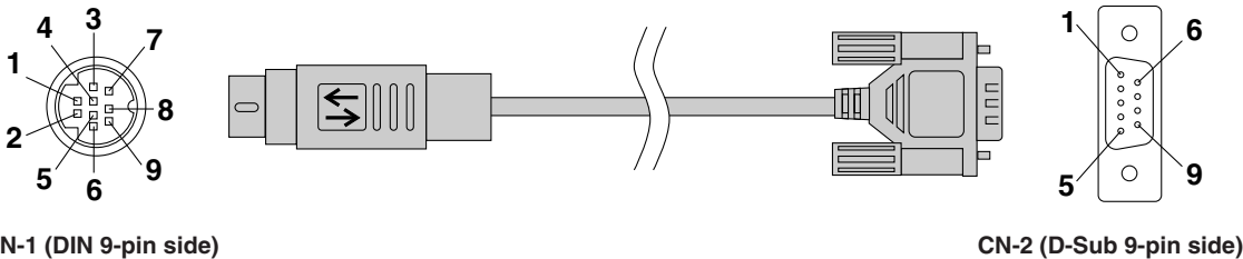
CN-1 (DIN 9-pin side)
