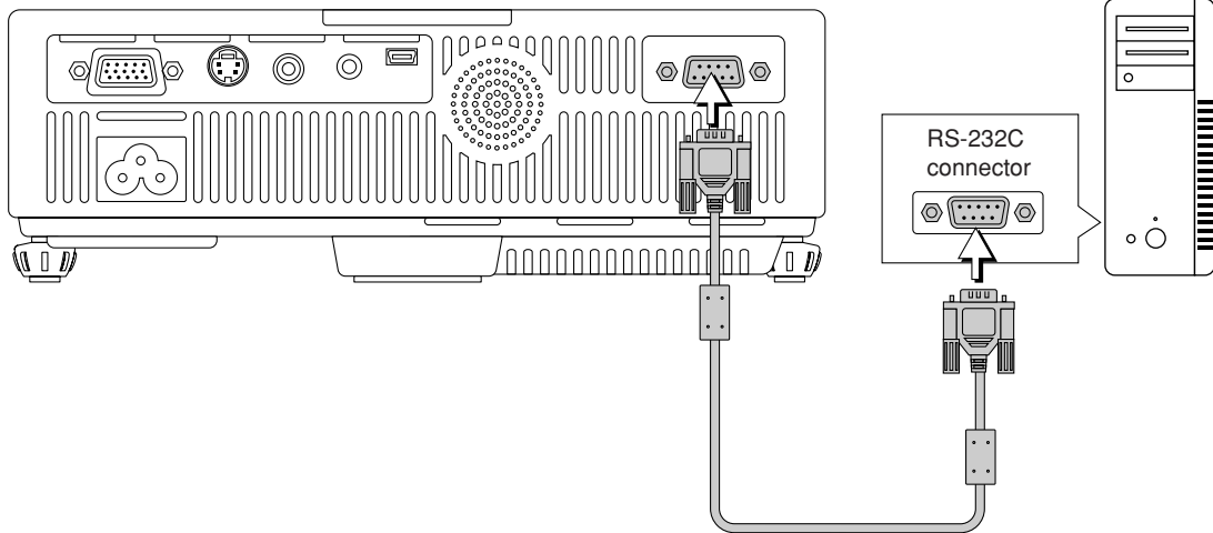
Serial cable (D-Sub 9-pin, straight) (commercially available)
