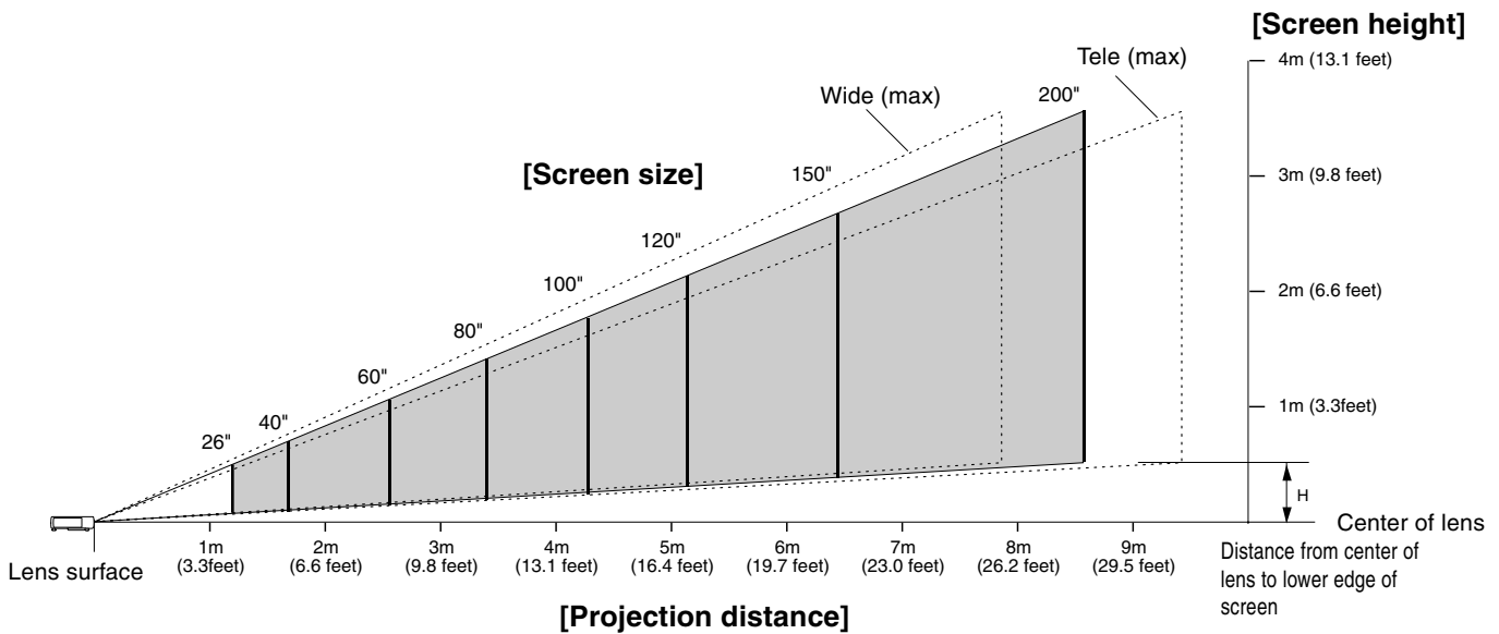
Projection distance and screen height for U3-1100Z
