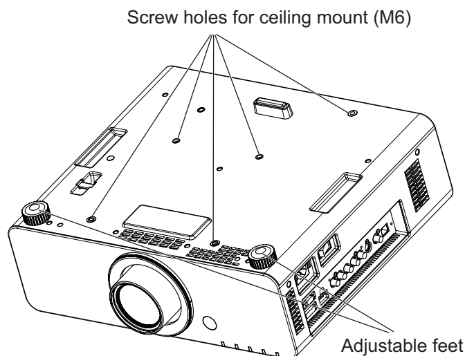
Fig. 1 The positions of screw holes for ceiling mount and adjustable feet
