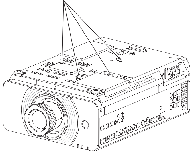
Ceiling mounting screws (M4)
