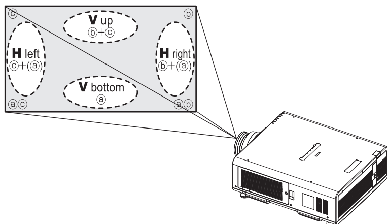
Figure 3 Relationship between the adjustment location and adjustment screws
