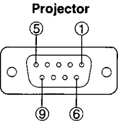
D-SUB 9-pin connector (female) seen from the outside
