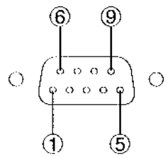
D-SUB 9-pin connector seen from outside
