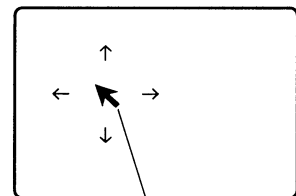
Mouse cursor
