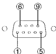
D-SUB 9-pin connector seen from outside
