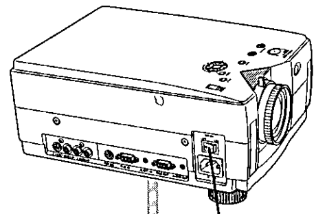
Main Power Switch
