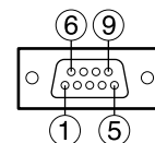
D-Sub 9-pin (female) external appearance
