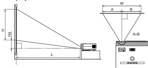
L : Between the screen and the front edge of the projector Hd : Height of the projected image
