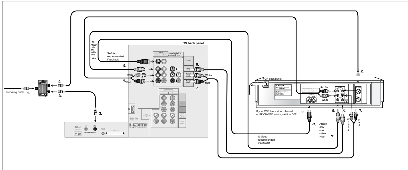
Figure 5. Connecting a VCR to an Antenna or Wall Outlet Cable
