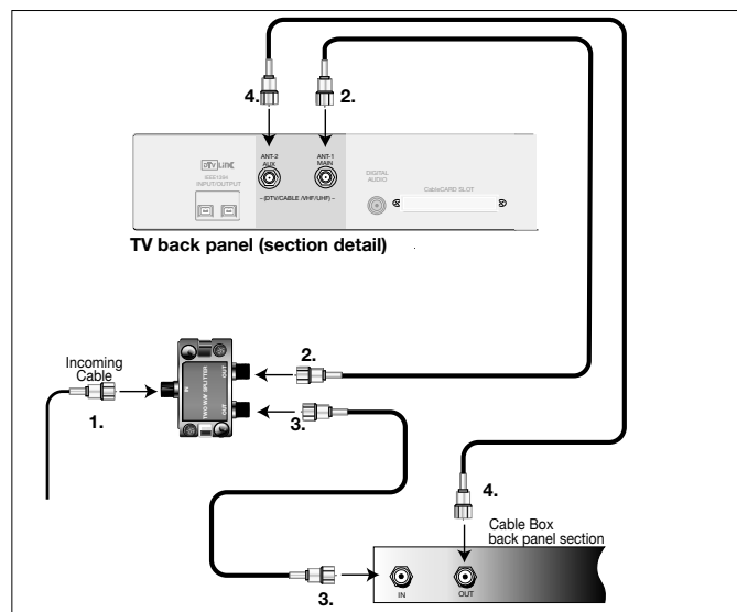
Figure 2. Connecting a Cable Box
