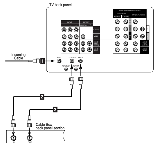
Figure 3. Connecting the cable box.
