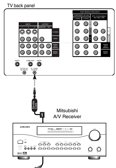
Figure 2. Connecting the Home Theater IR System.
