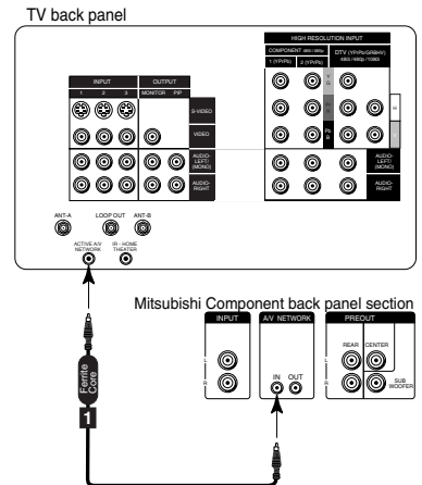
Figure 1. Connecting the Active A/V Network.
