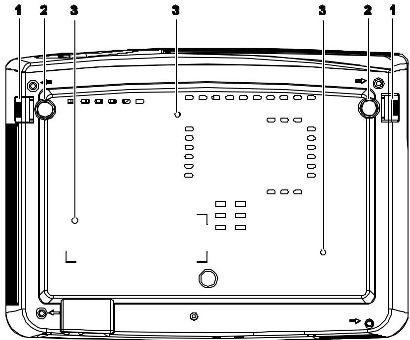
Bottom view
