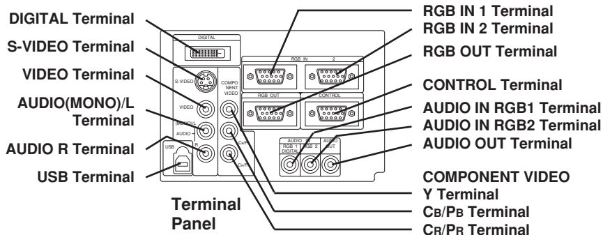
Rear/Left View
