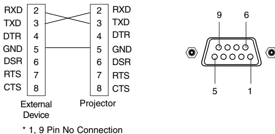
<Fig.1, RS-232 Interface Cable>
