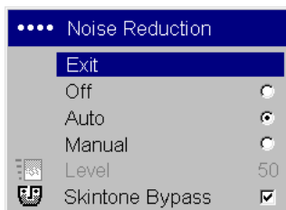
Noise reduction
