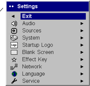
Settings menu
