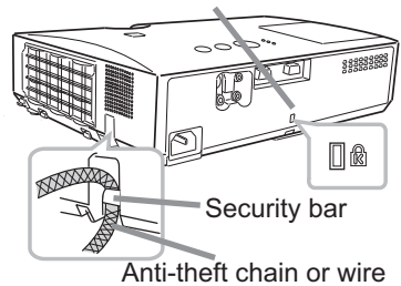
Security slot
