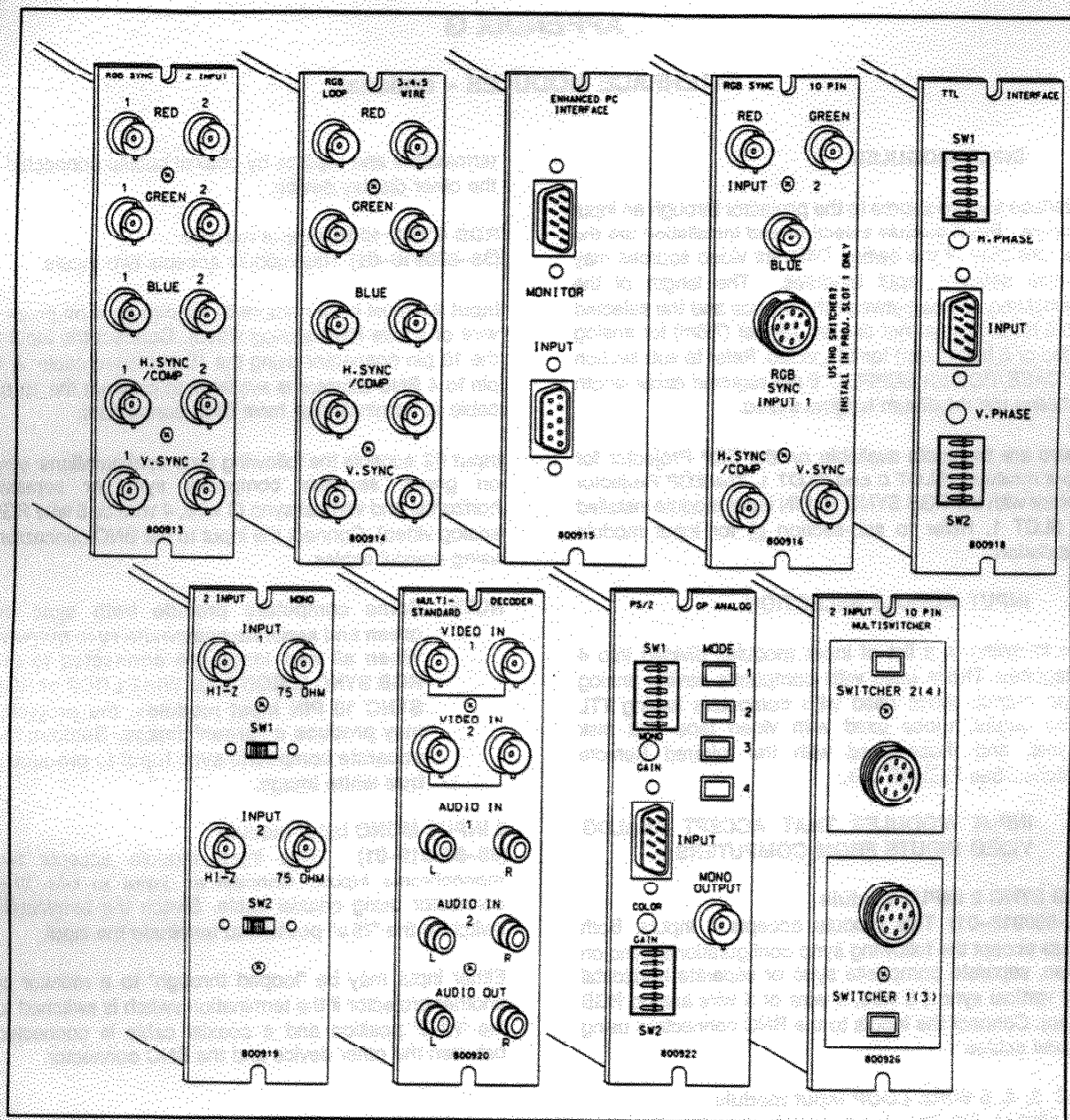
FIGURE G-1. Interface Input Modules
