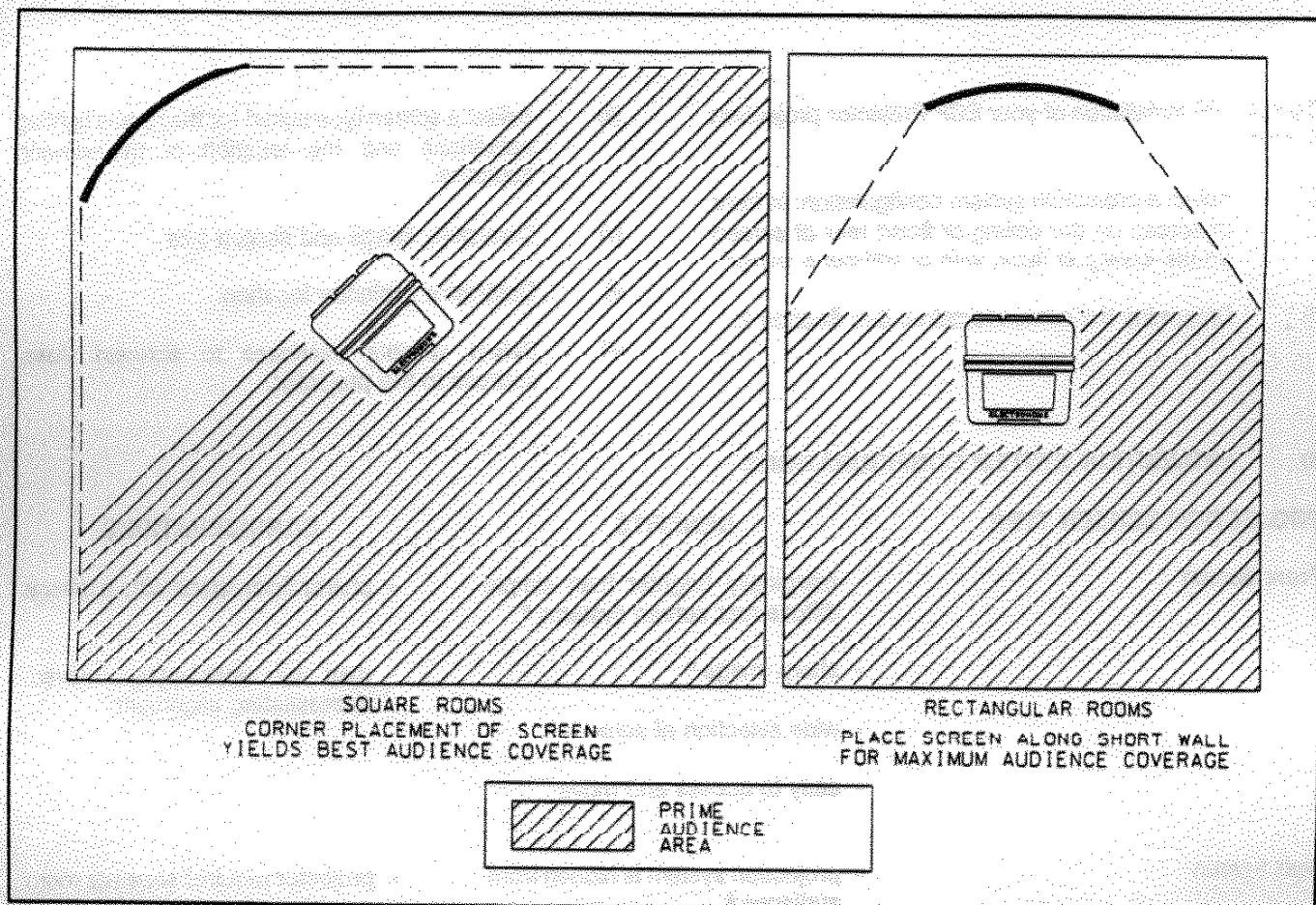
FIGURE D-1. Screen Locations for Maximum Audience Coverage
