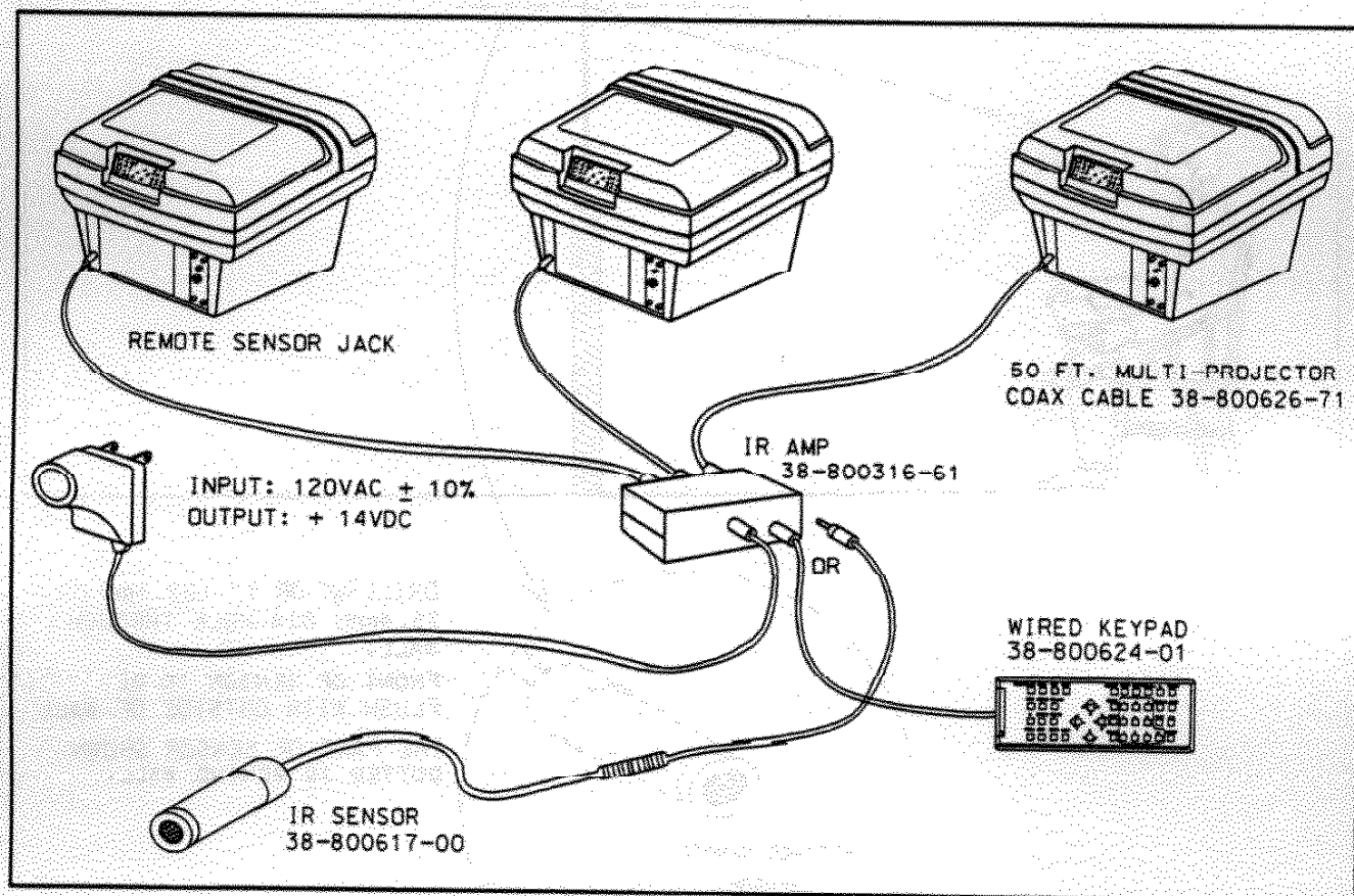
FIGURE 3-4. Multiprojector Systems
