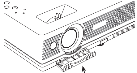
Air filter Pull horizontally and remove.
