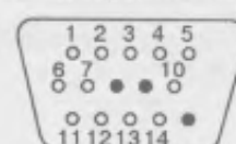
Computer HD-DB15 (Male)
