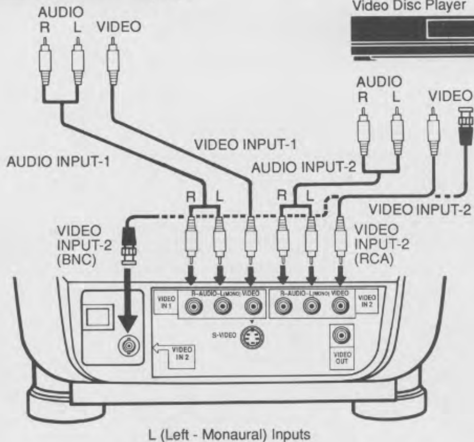
Video Disc Player
